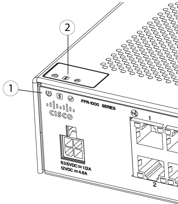
图 8: 状态 LED
