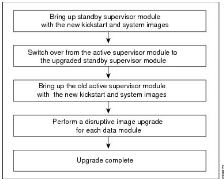
Figure 8: ISSU Process
