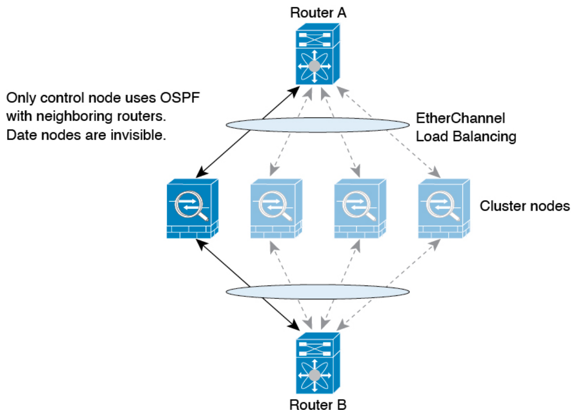
Figure 204: Dynamic Routing in Spanned EtherChannel Mode
