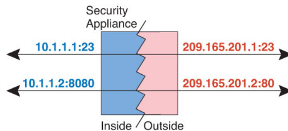
Figure 365: Typical Static NAT with Port Translation Scenario
