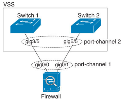
Figure 287: Connecting to a VSS/vPC
