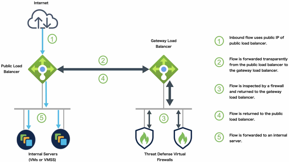
Figure 246: Inbound Traffic Use Case and Topology with GWLB
