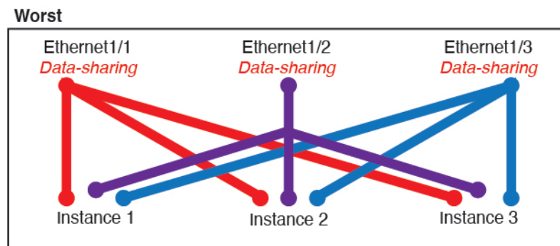
Figure 105: Worst: Shared Parent Interfaces
