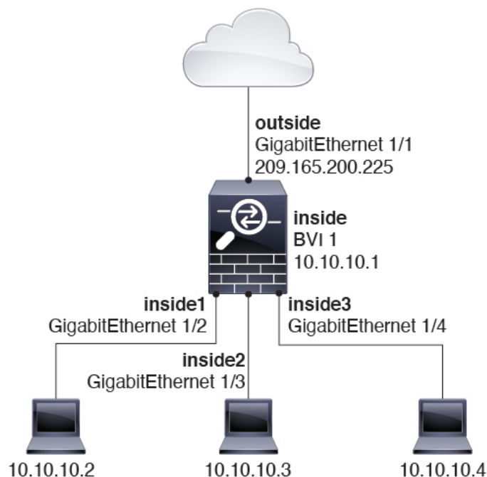
Figure 89: Routed Firewall Network with an Inside Bridge Group and an Outside Routed Interface
