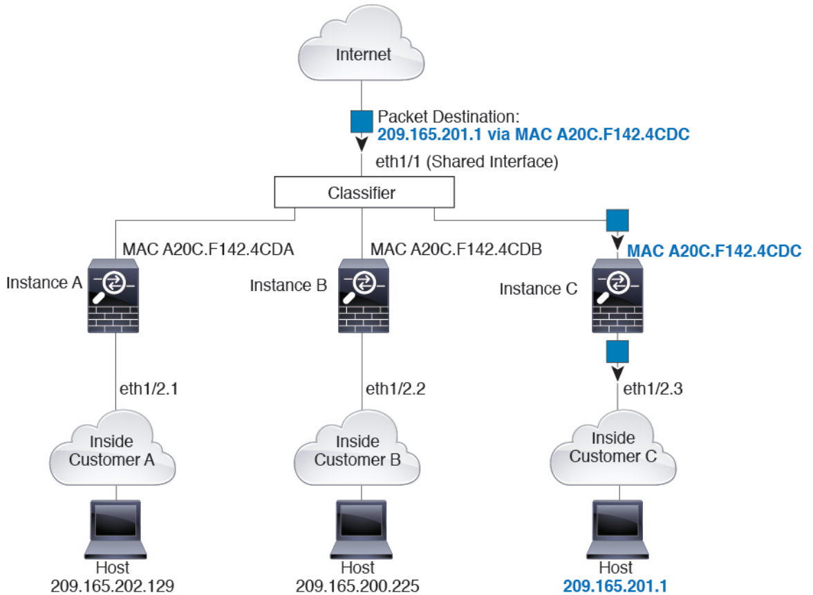
Figure 106: Packet Classification with a Shared Interface Using MAC Addresses
