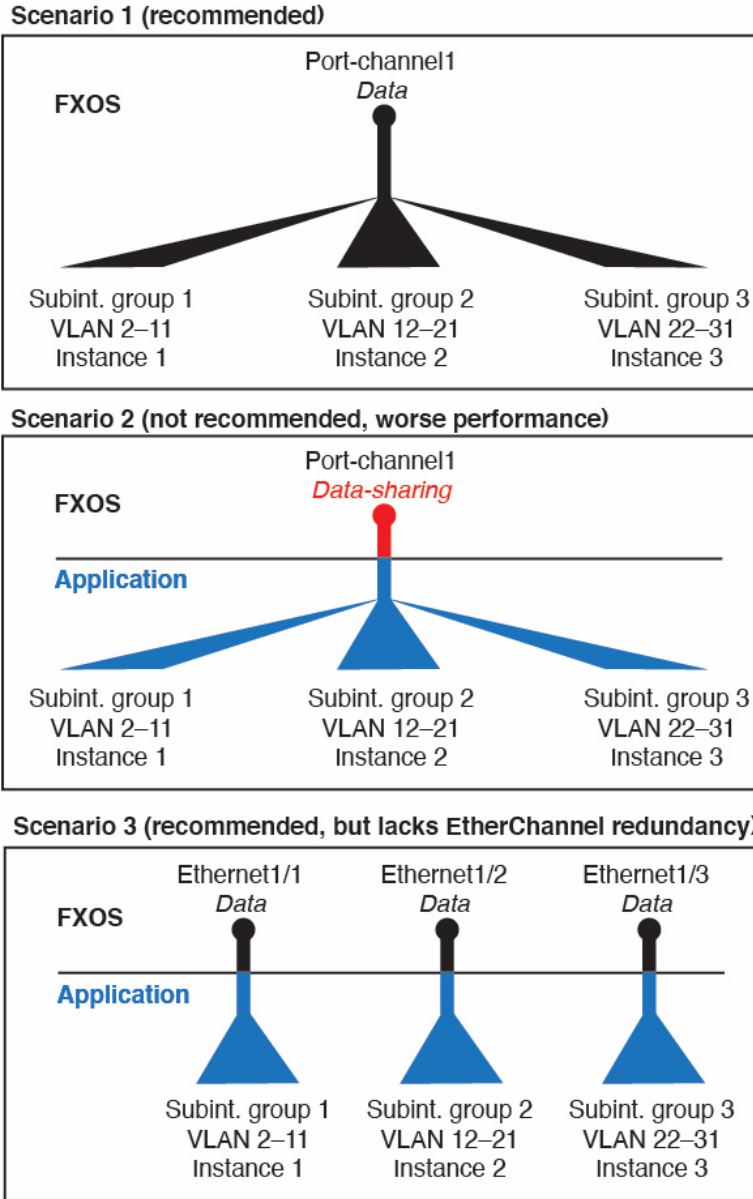
Figure 101: VLANs in the Chassis vs. the Instance
