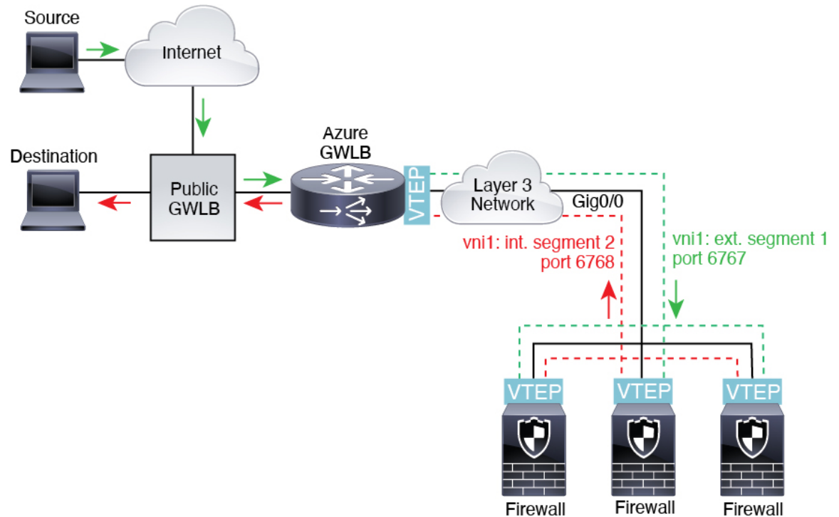
Figure 345: Azure Gateway Load Balancer with Paired Proxy
