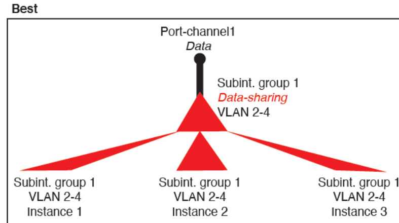
Figure 102: Best: Shared Subinterface Group on One Parent
