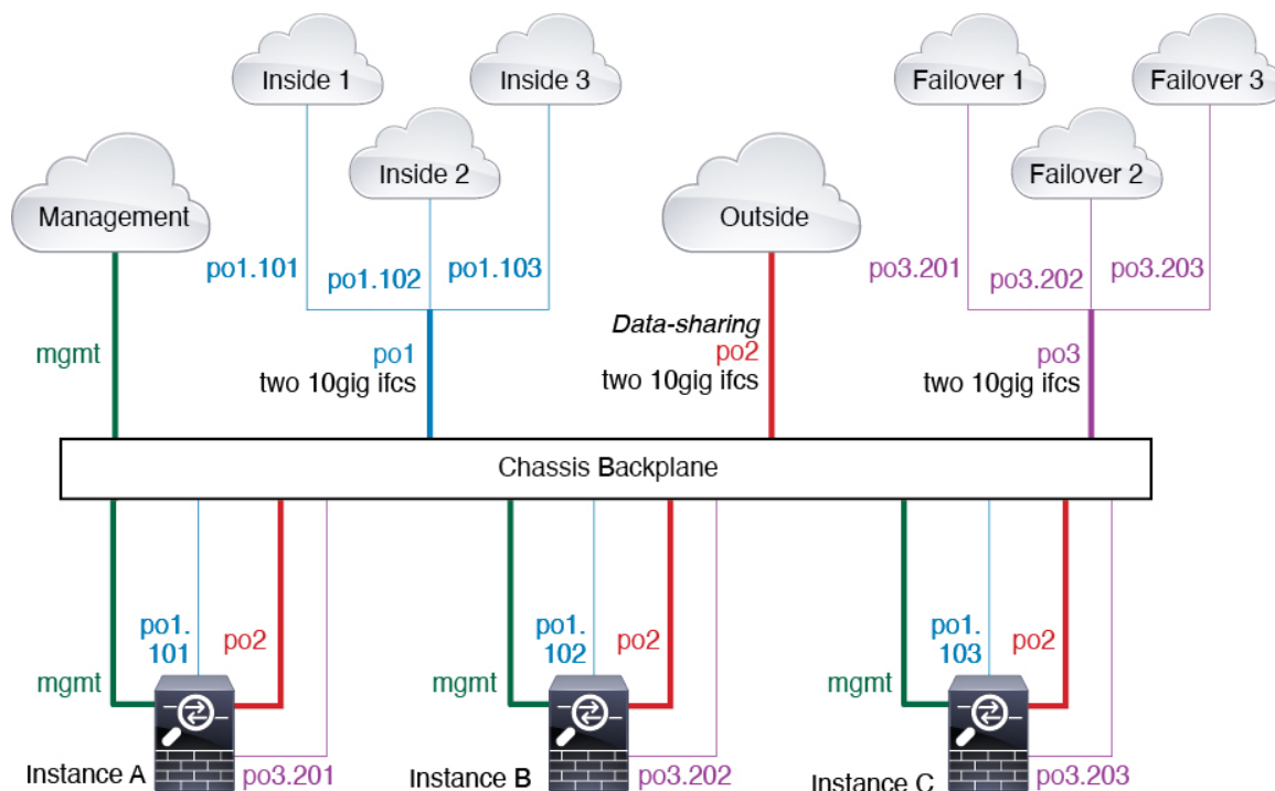
Figure 111: Typical Multi-Instance Deployment
