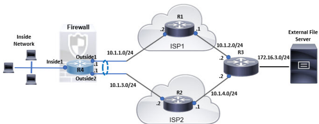
Figure 383: Configuration Example for ECMP
