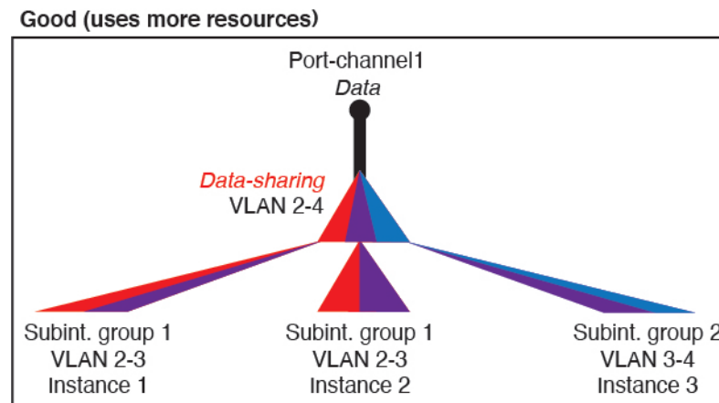
Figure 103: Good: Sharing Multiple Subinterface Groups on One Parent
