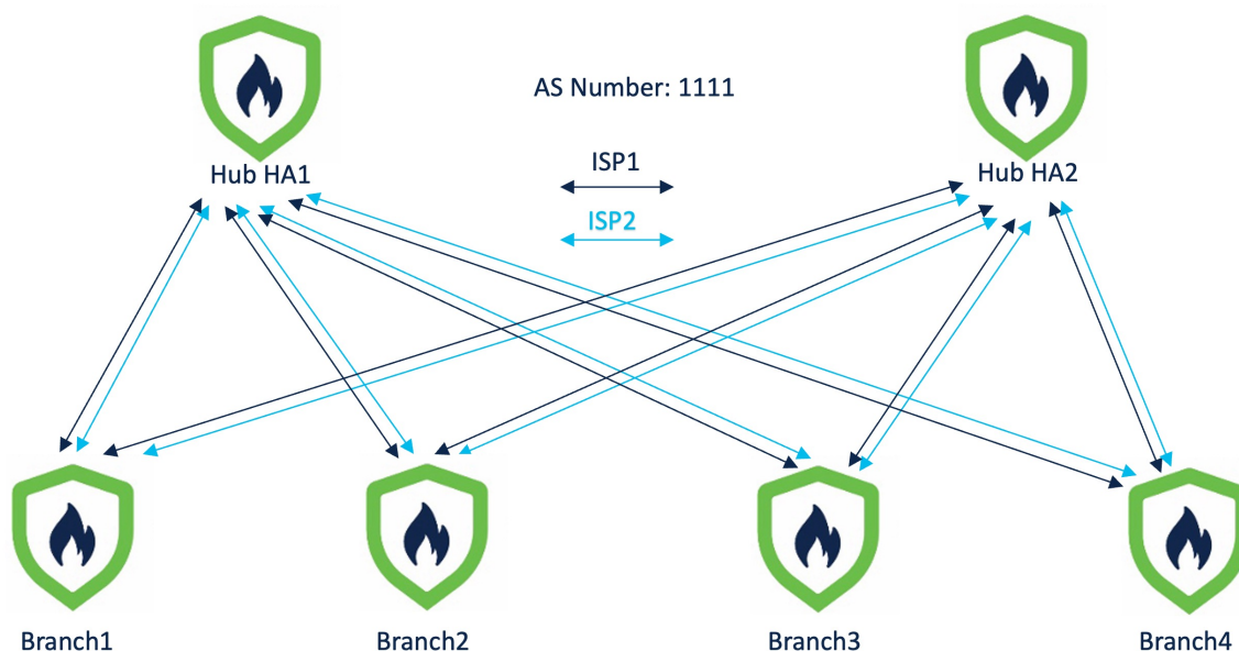
Figure 411: Dual ISP Topology with Two Hubs and Four Spokes in the Same Region
