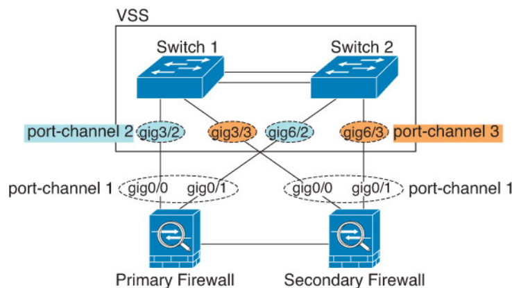
Figure 288: Active/Standby Failover and VSS/vPC
