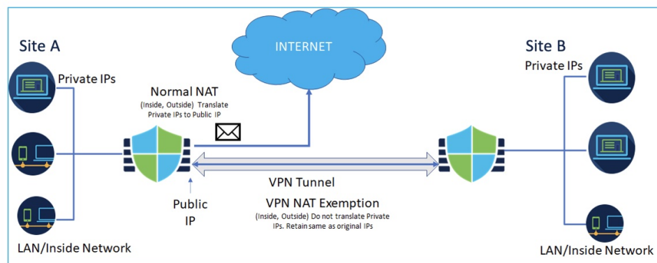
Figure 360: Site-to-site VPN Topology with NAT Exemption
