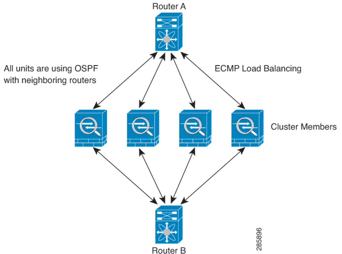
Figure 379: Dynamic Routing in Individual Interface Mode
