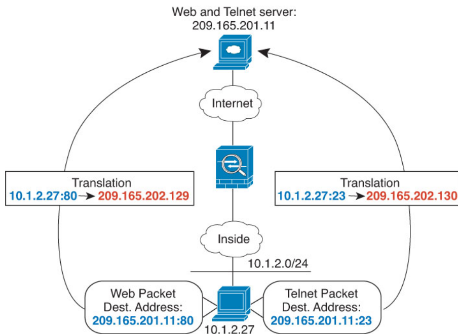
Figure 376: Manual NAT with Different Destination Ports
