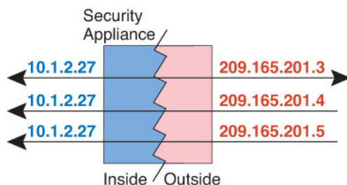
Figure 366: One-to-Many Static NAT
