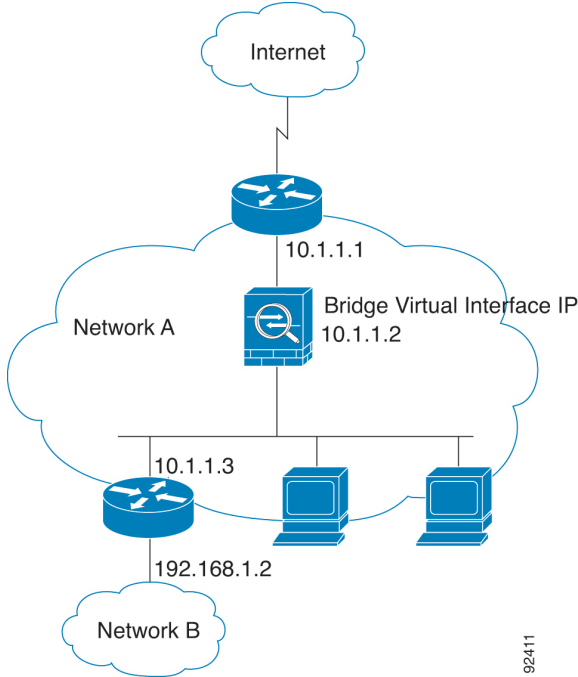
Figure 87: Transparent Firewall Network
