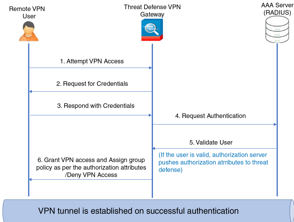
Figure 403: Remote Access VPN Group Policy Selection by AAA Server
