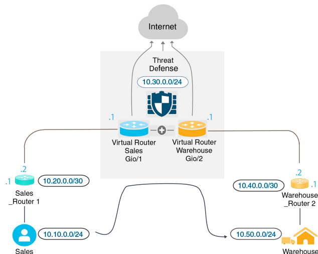
Figure 380: Interconnecting Two Virtual Routers - An Example
