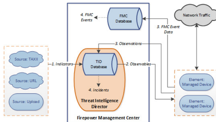
Figure 416: Management Center Data Flow
