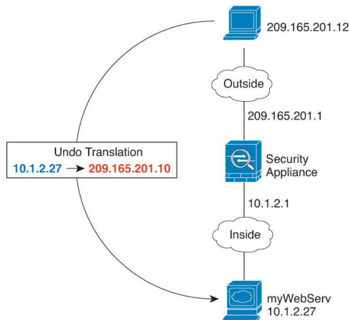
Figure 371: Static NAT for an Inside Web Server
