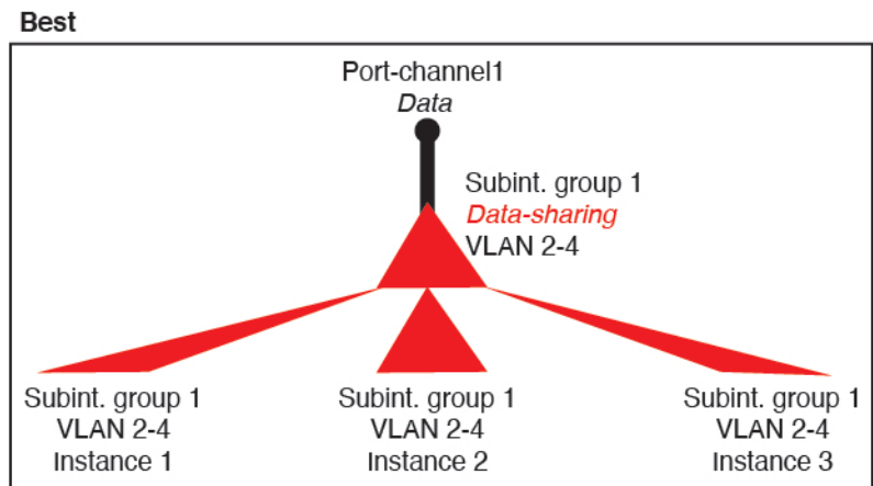
Figure 92: Best: Shared Subinterface Group on One Parent
