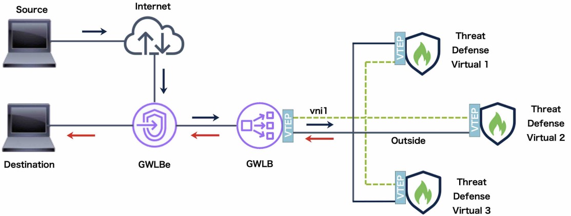
Figure 240: Geneve Single-Arm Proxy
