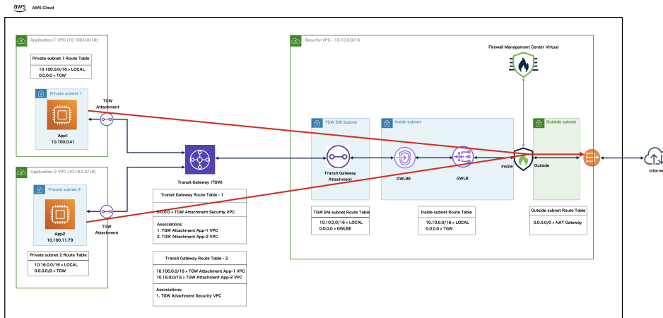
Figure 344: Geneve Dual-Arm Proxy: Egress Traffic from Multiple VPCs
