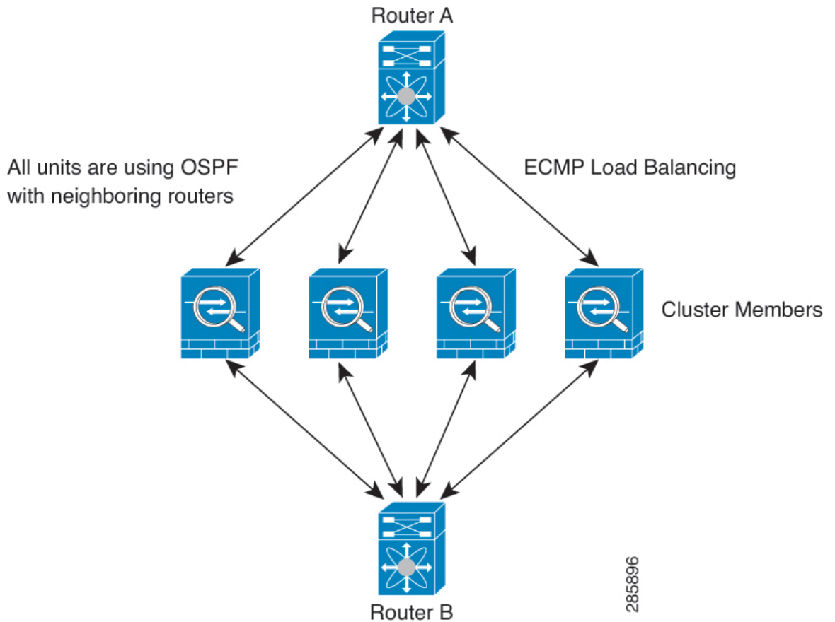
Figure 238: Dynamic Routing in Individual Interface Mode
