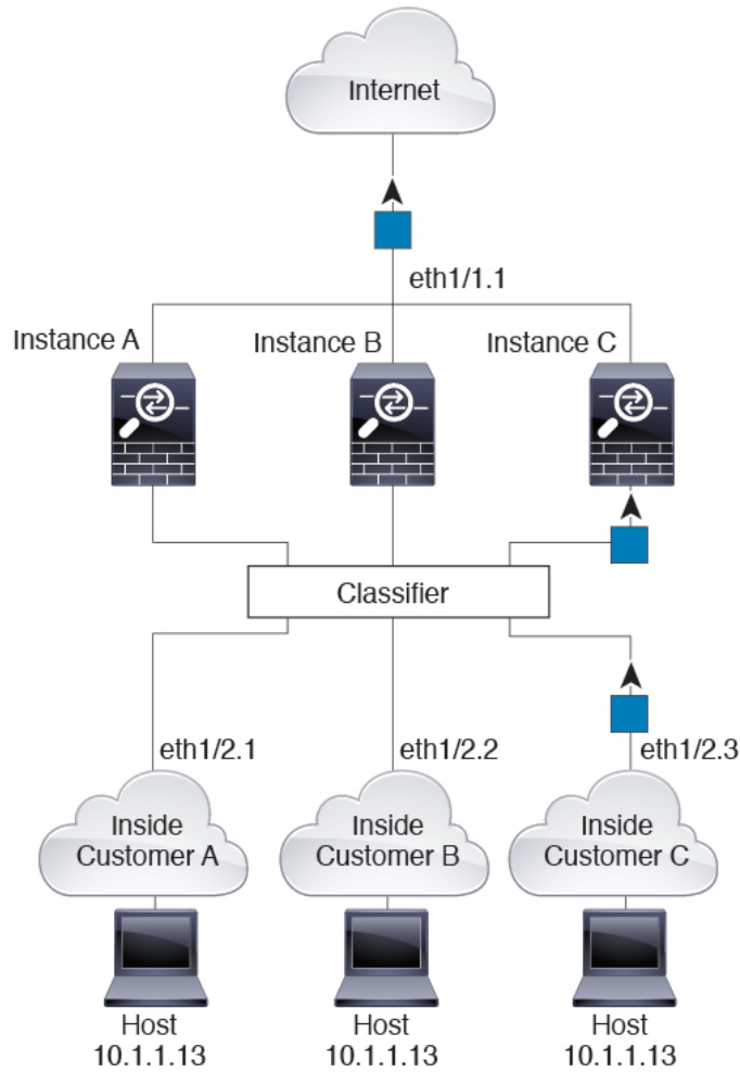
Figure 97: Incoming Traffic from Inside Networks
