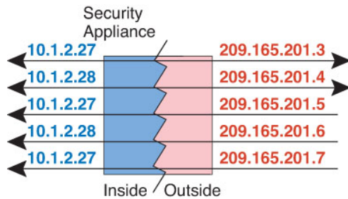
Figure 368: Few-to-Many Static NAT
