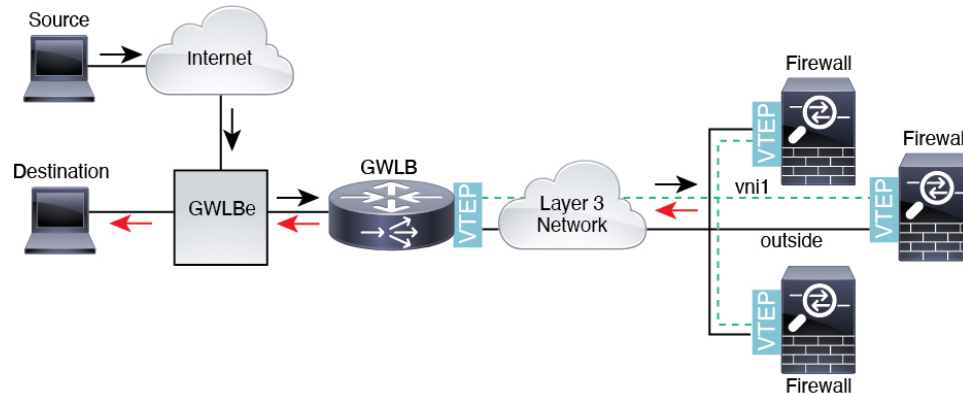
Figure 342: Geneve Single-Arm Proxy
