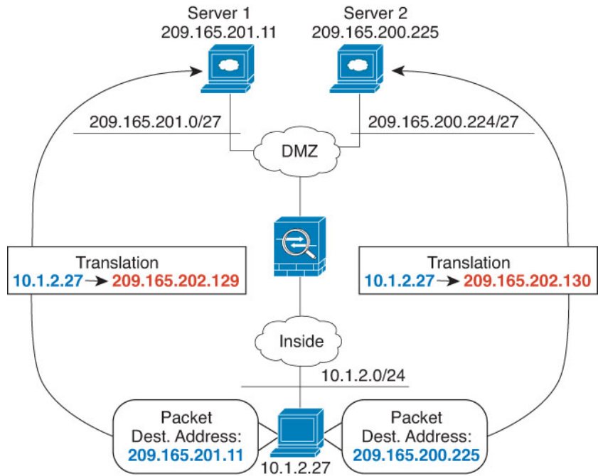
Figure 375: Manual NAT with Different Destination Addresses
