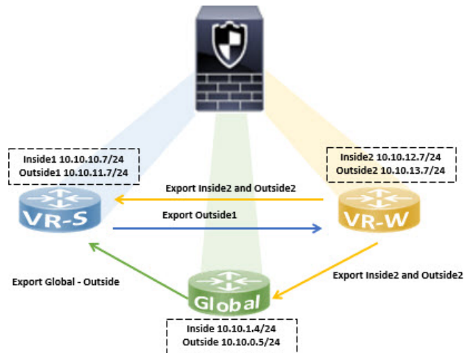
Figure 382: Interconnect Virtual Routers using BGP Settings
