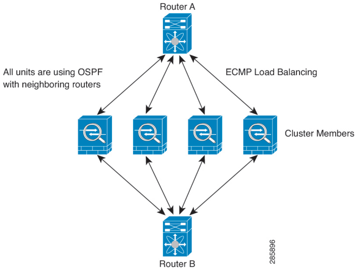
Figure 205: Dynamic Routing in Individual Interface Mode
