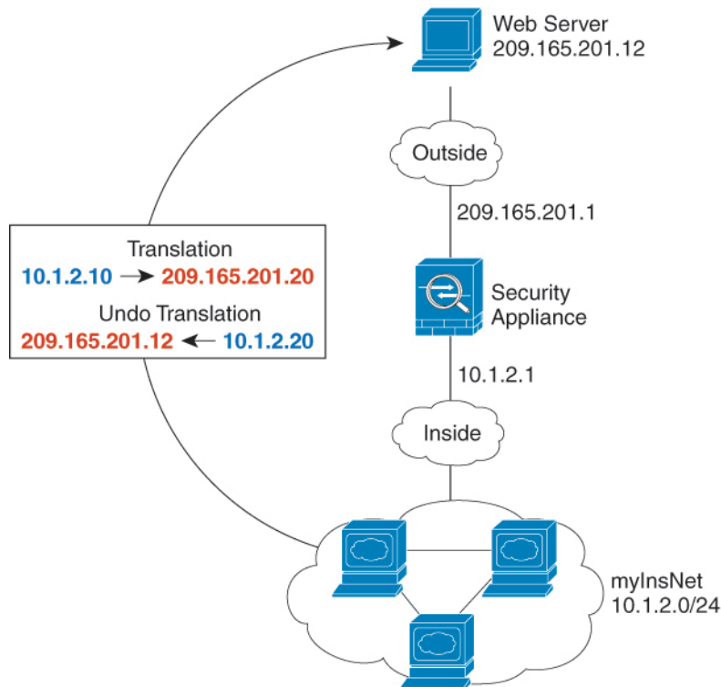
Figure 372: Dynamic NAT for Inside, Static NAT for Outside Web Server
