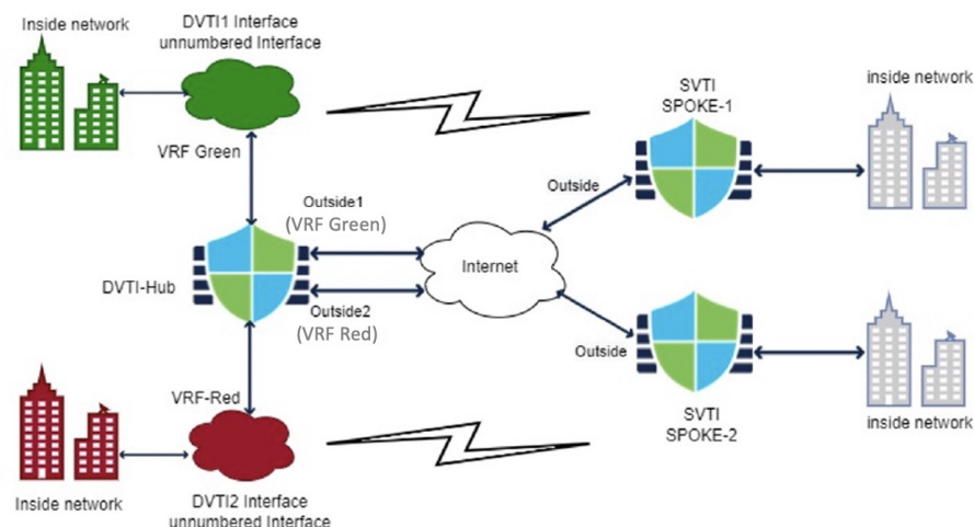
Figure 381: Site-to-Site VPNs with Multiple Virtual Routers and Dynamic VTI
