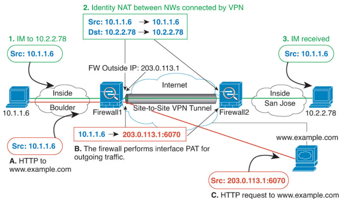
Figure 377: Interface PAT and Identity NAT for Site-to-Site VPN
