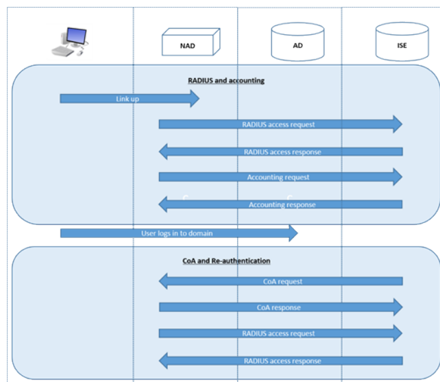
Figure 19: Easy Connect Enforcement Mode Detailed Flow
