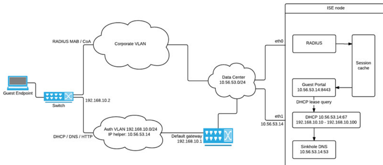
Figure 30: Auth VLAN Configured with IP Helper
