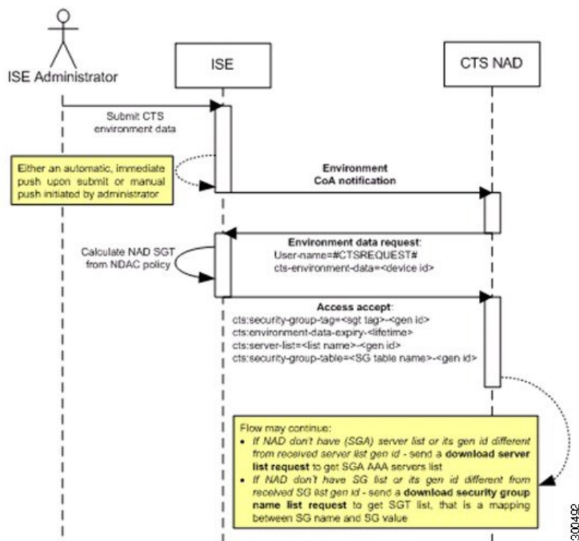
Figure 48: Environment CoA Notification Flow
