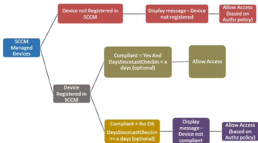
Figure 34: SCCM Workflow
