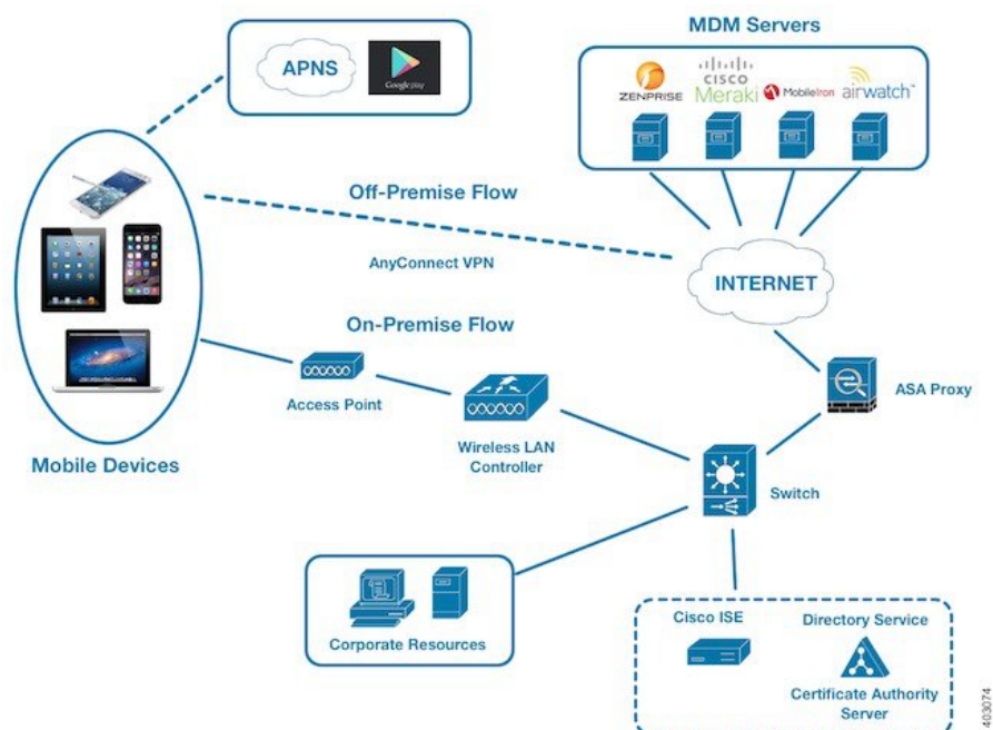
Figure 31: MDM Interoperability with Cisco ISE
