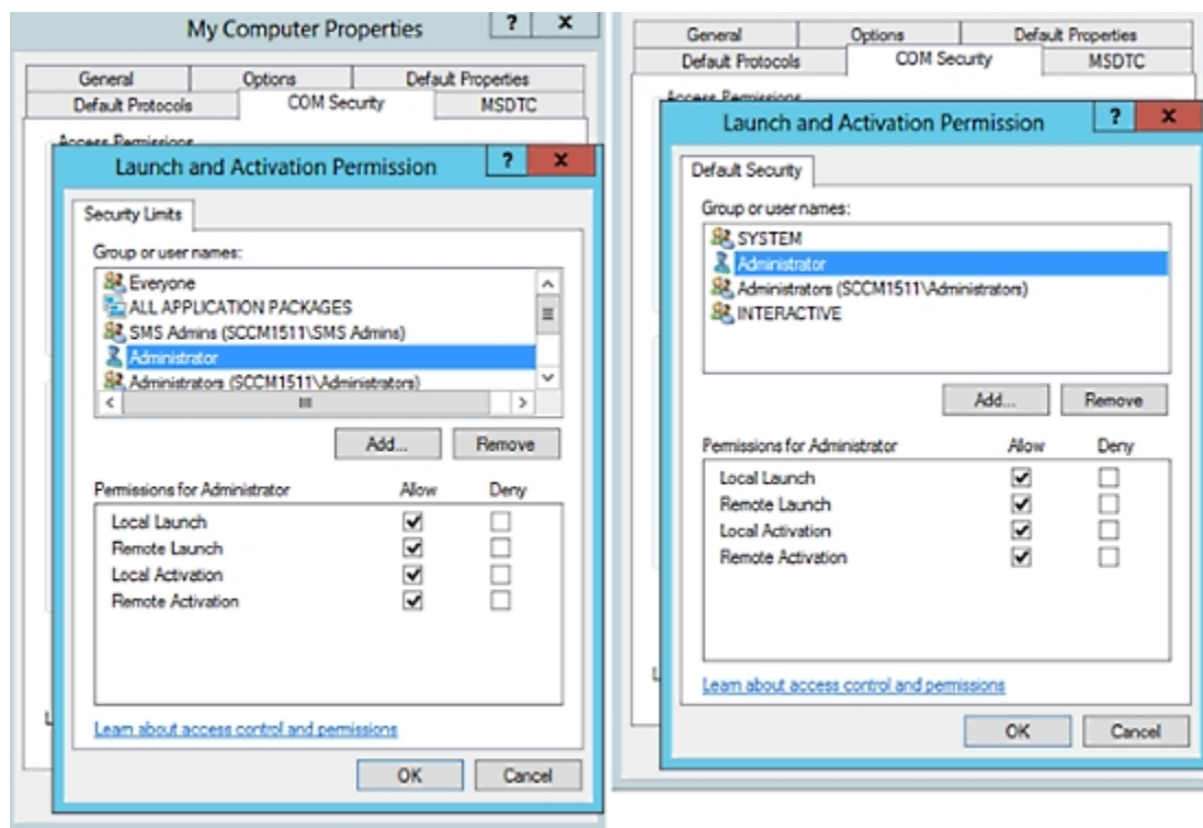
Figure 17: Local and Remote Accesses for Launch and Activation Permissions
