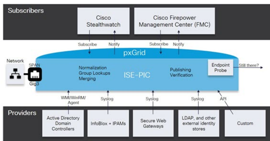
Figure 21: High Level Flow
