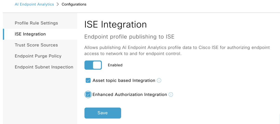
Figure 40: ISE Integration Settings in Cisco AI Endpoint Analytics
