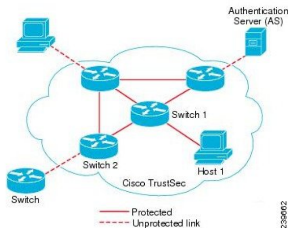
Figure 46: TrustSec Architecture
