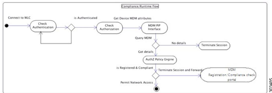
Figure 32: The MDM Process Flow in Cisco ISE
