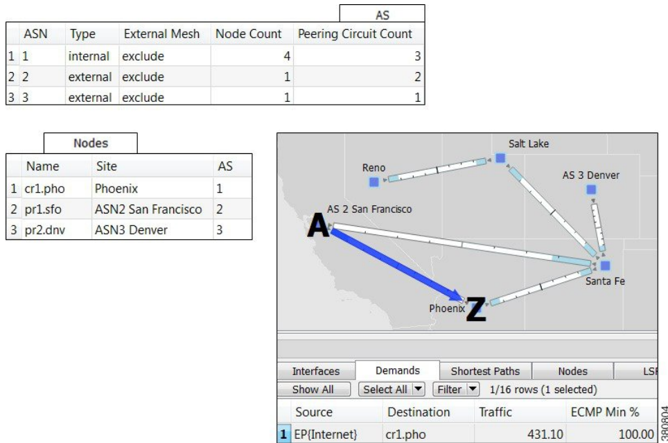
Figure 8: Example Failover to a Different External AS
