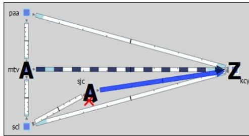
Figure 3: Example Failover for Multiple Data Centers
