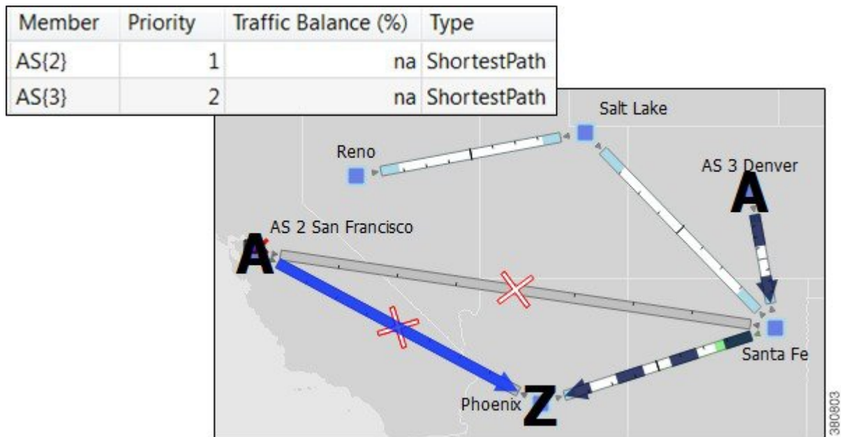
Figure 8: Example Failover to a Different External AS
