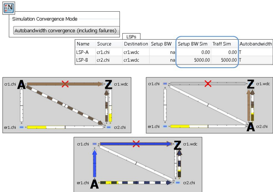
Figure 55: Example Autobandwidth Convergence Including Failures
