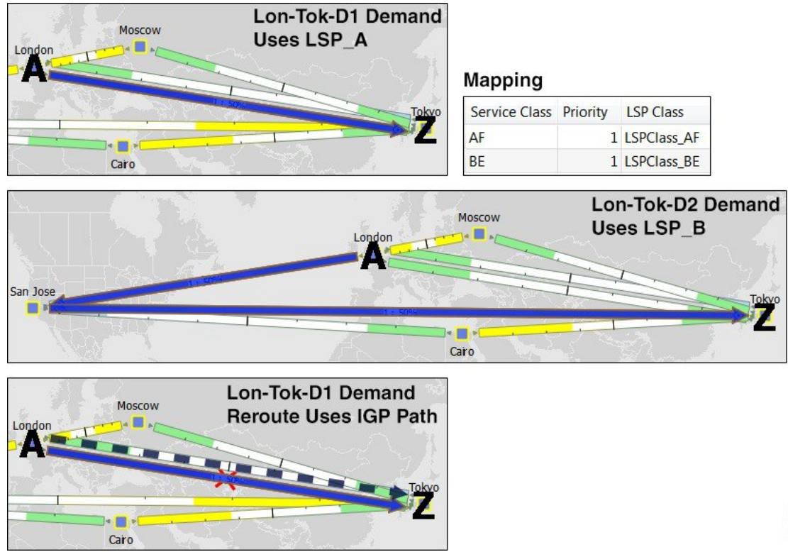
Figure 36: Example Reroute Around Failure Using IGP Path
