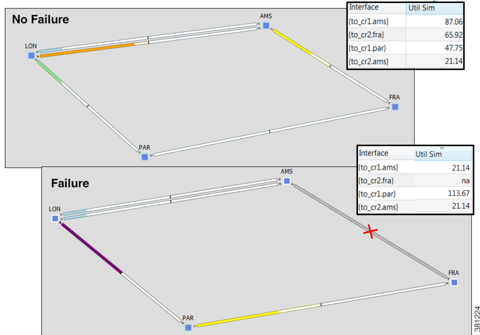
Figure 5-1 Failed Circuit
