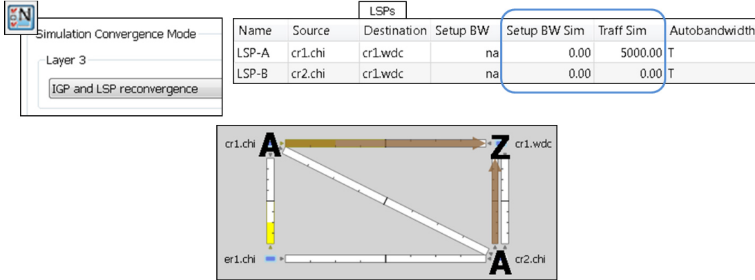
Figure 10-13 Example LSP Routing Using IGP and LSP Reconvergence and Using Autobandwidth Convergence
