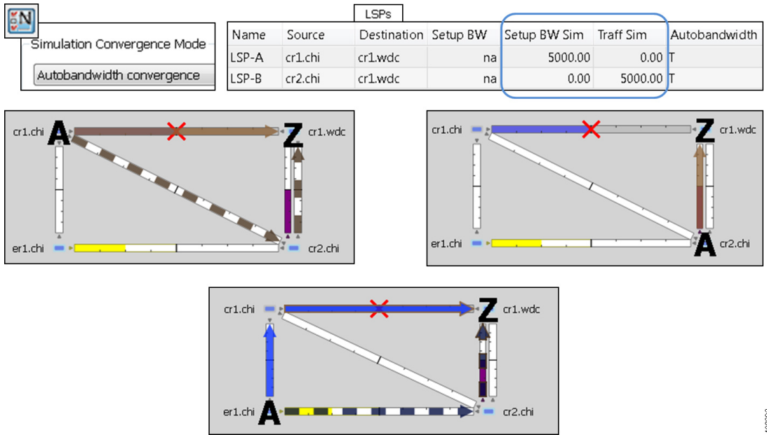
Figure 10-14 Example Autobandwidth Convergence with Failures
