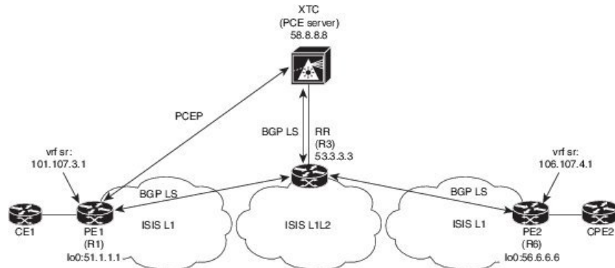
Figure 2: ODN Auto-Tunnel Setup
