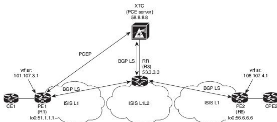
Figure 16: ODN Auto-Tunnel Setup
