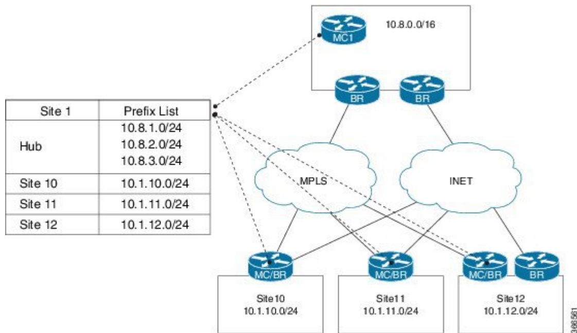
Figure 11: Pfrv3-discovery-site-prefix.png
