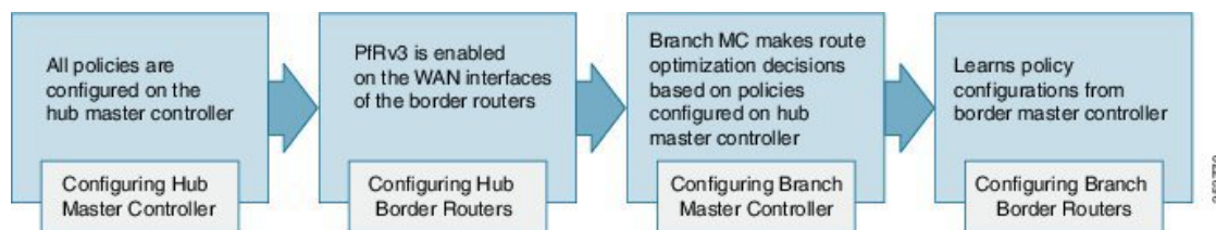
Figure 2: PfRv3 Workflow
