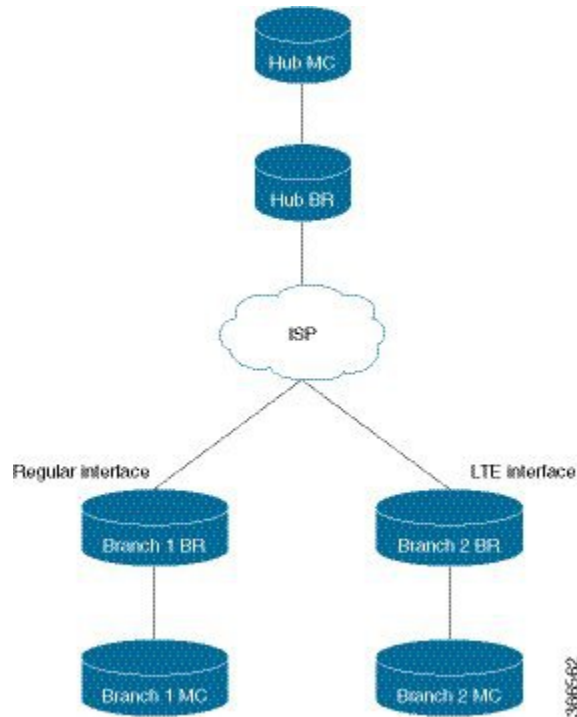
Figure 13: Per Interface Probe Tuning—Sample Topology
