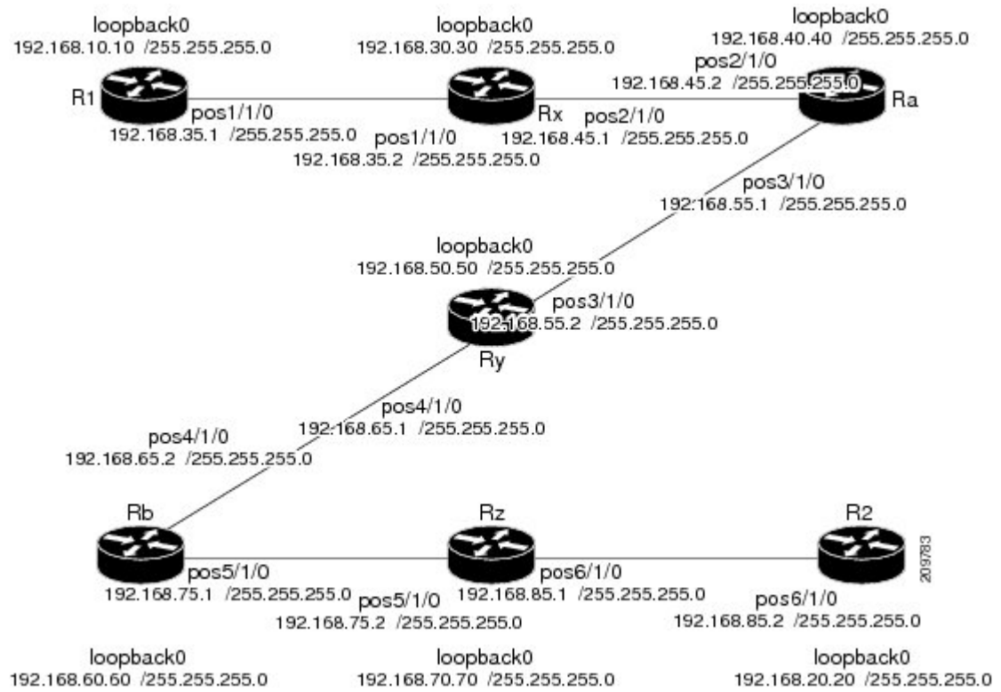
Figure 7: Router Topology
