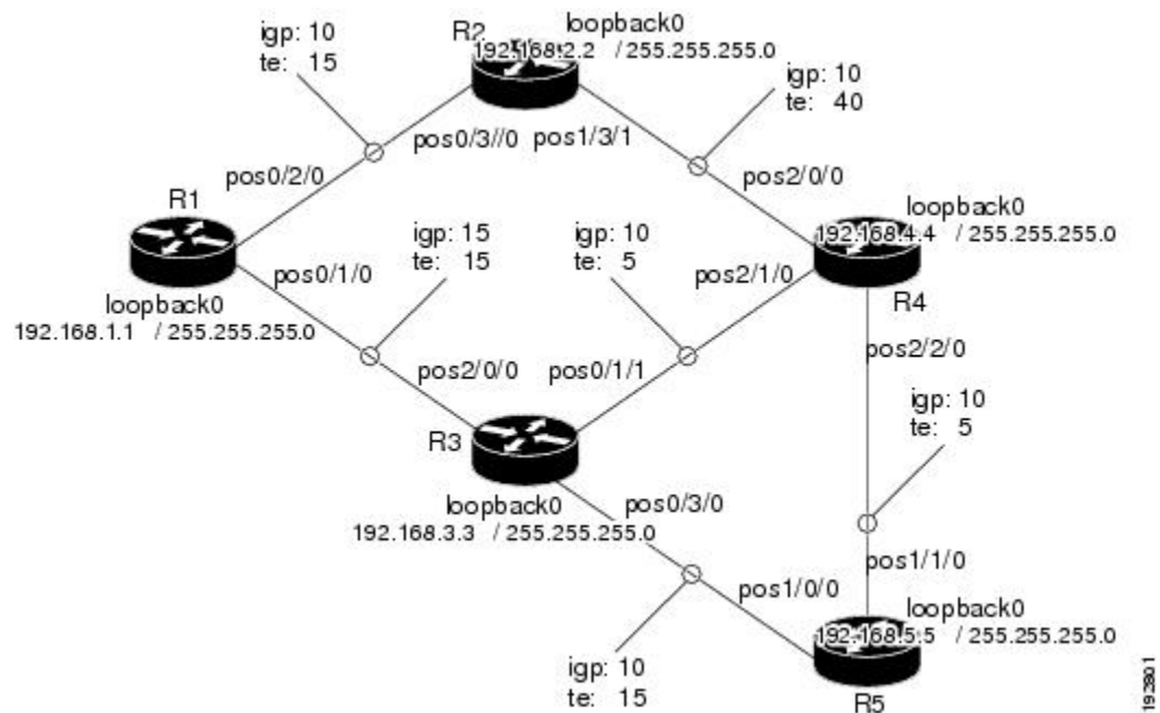
Figure 4: Network Topology
