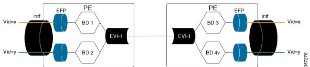
Figure 54: VLAN-Aware Bundle Service Interface
