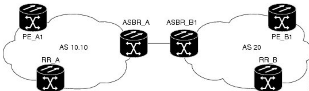
Figure 23: L2VPN VPLS Inter-AS Option B Topology Used for Configuration Example
