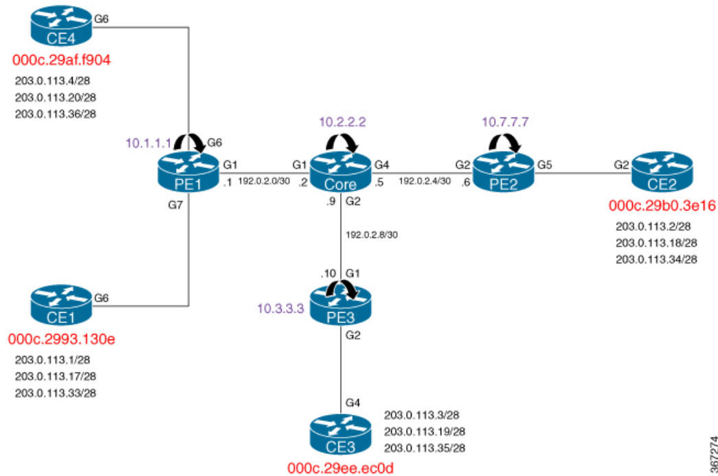
Figure 49: EVPN Single Homing
