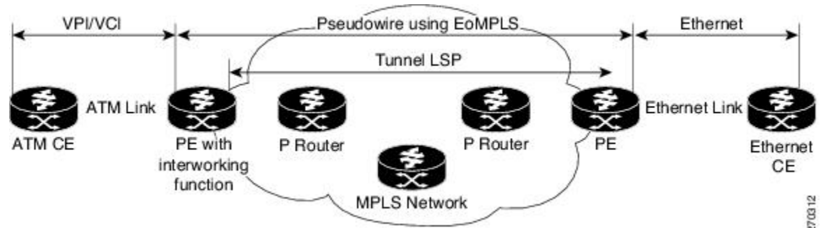
Figure 10: Network Topology for ATM-to-Ethernet AToM Bridged Interworking
