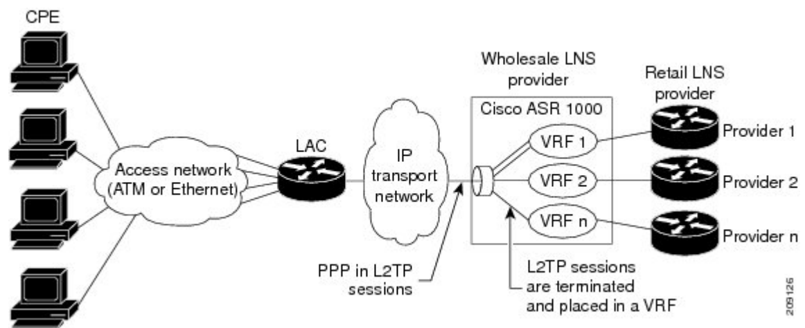
Figure 27: Terminating and Forwarding Sessions from the LAC
