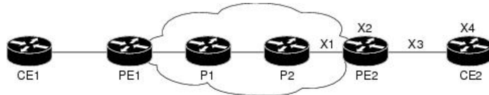
Figure 28: Points of Potential Failure in an L2VPN Network
