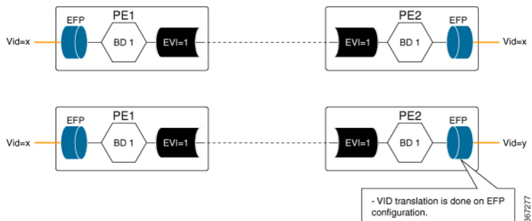
Figure 46: VLAN-Based Service Interface
