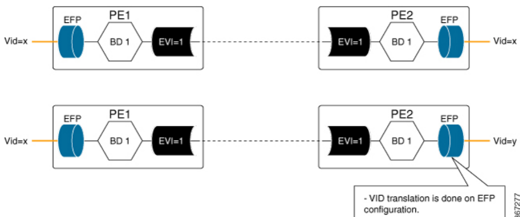
Figure 52: VLAN-Based Service Interface
