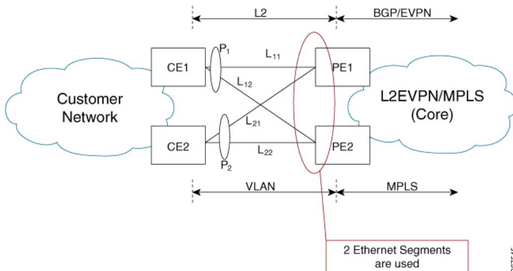
Figure 50: EVPN Multihoming Topology
