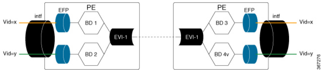
Figure 48: VLAN-Aware Bundle Service Interface
