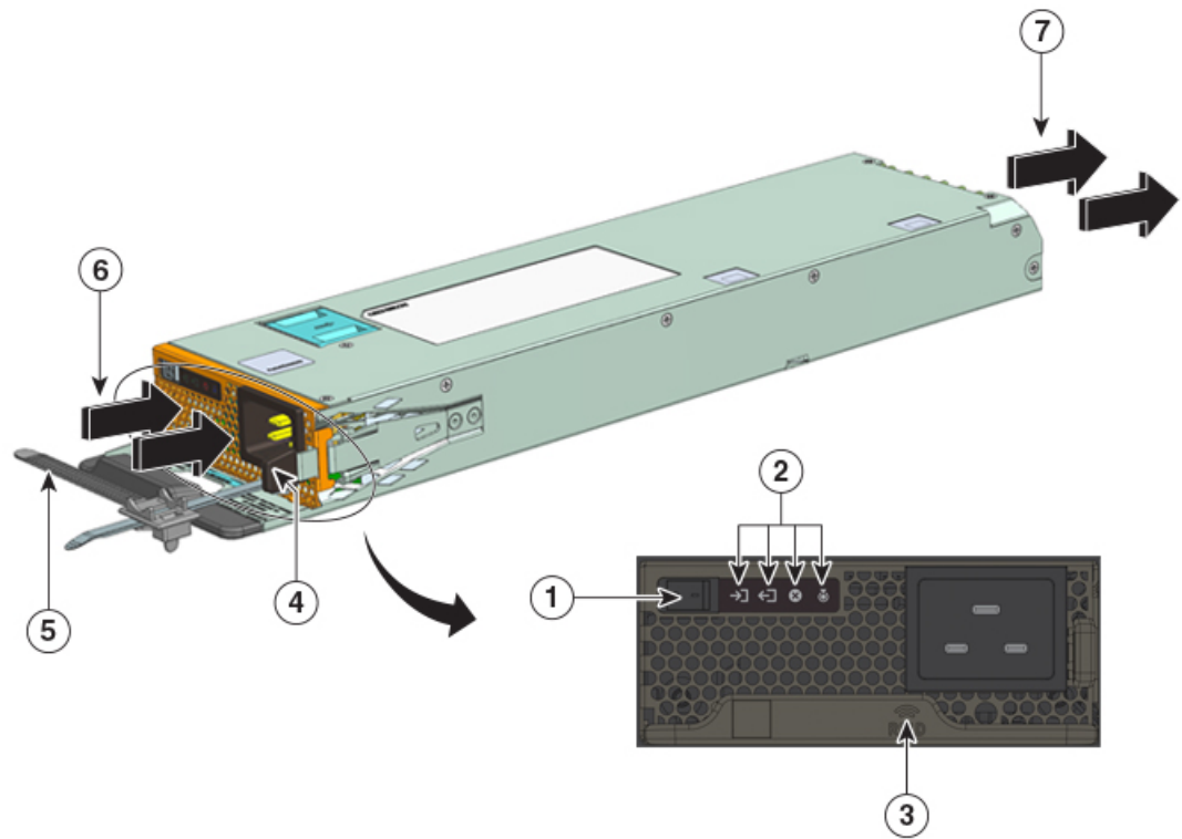
图 3: C9400-PWR-3200ACT
