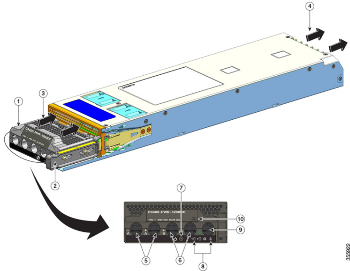
图 4: C9400-PWR-3200DC
