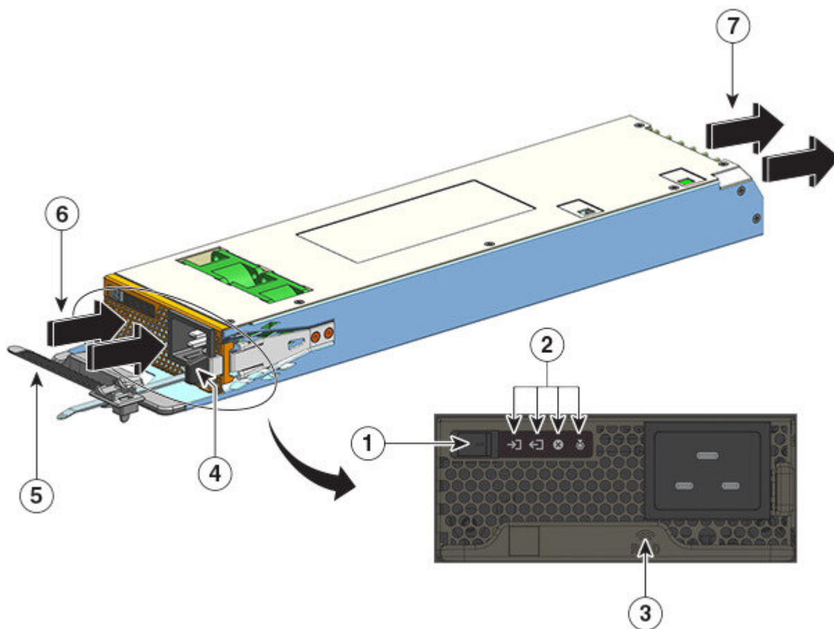
图 2: C9400-PWR-3200AC
