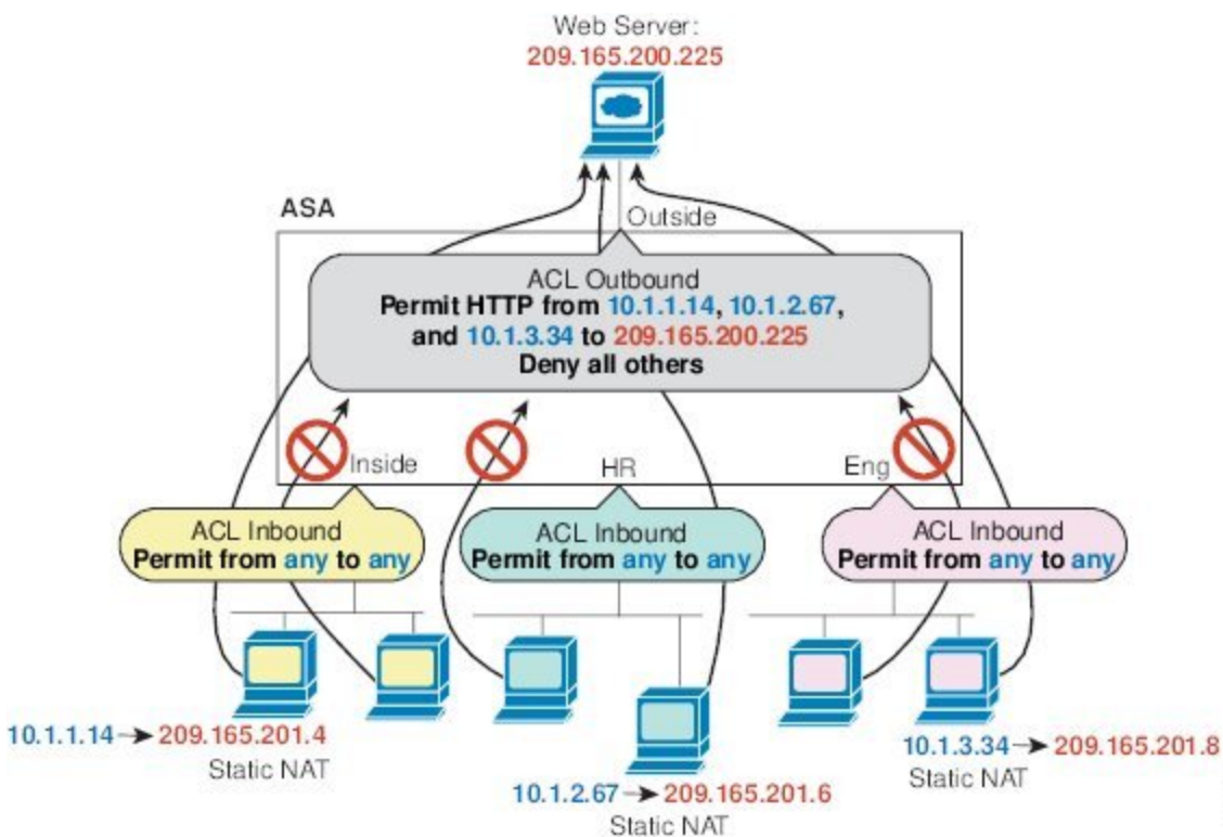
図 1: Outbound ACL
