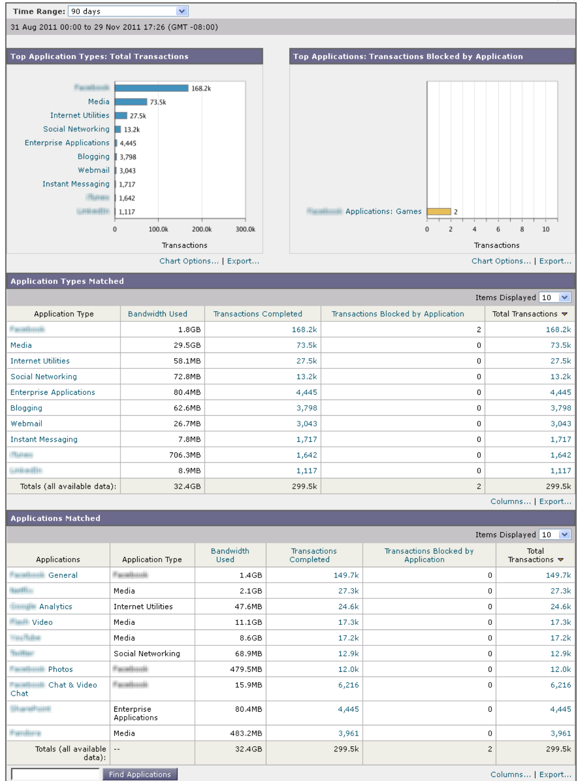
図 5-8 [Application Visibility] ページ Application Visibility
