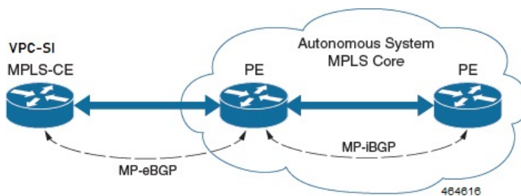
Figure 19: VPC-SI MPLS-CE to PE
