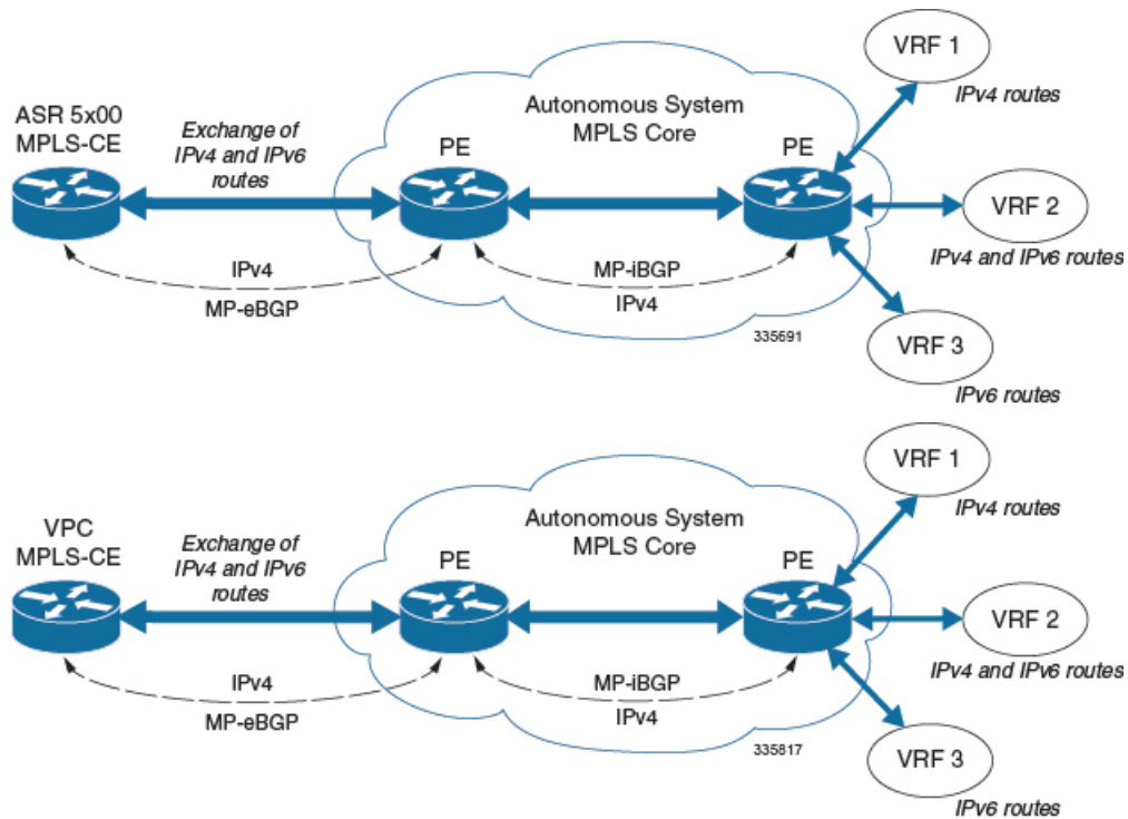
Figure 26: VPNv6 Sample Configuration
