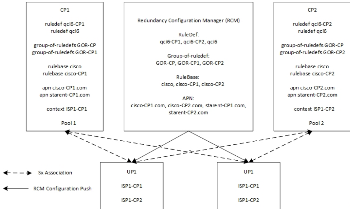
Figure 27: Sample RCM Configuration of Two CPs Communicating with Two UPs
