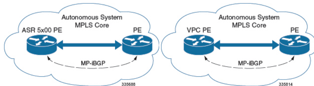
Figure 23: VPC-SI as a PE
