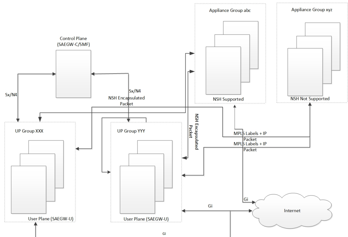
Figure 39: NSH Traffic Steering Architecture—Standalone Mode
