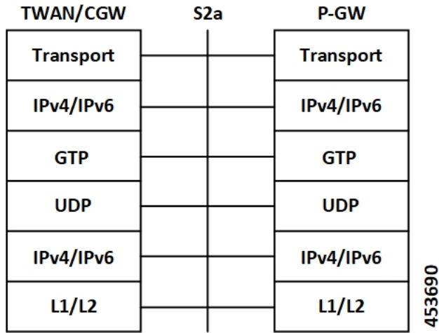
Figure 43: Protocols Supported on the S2a Interface
