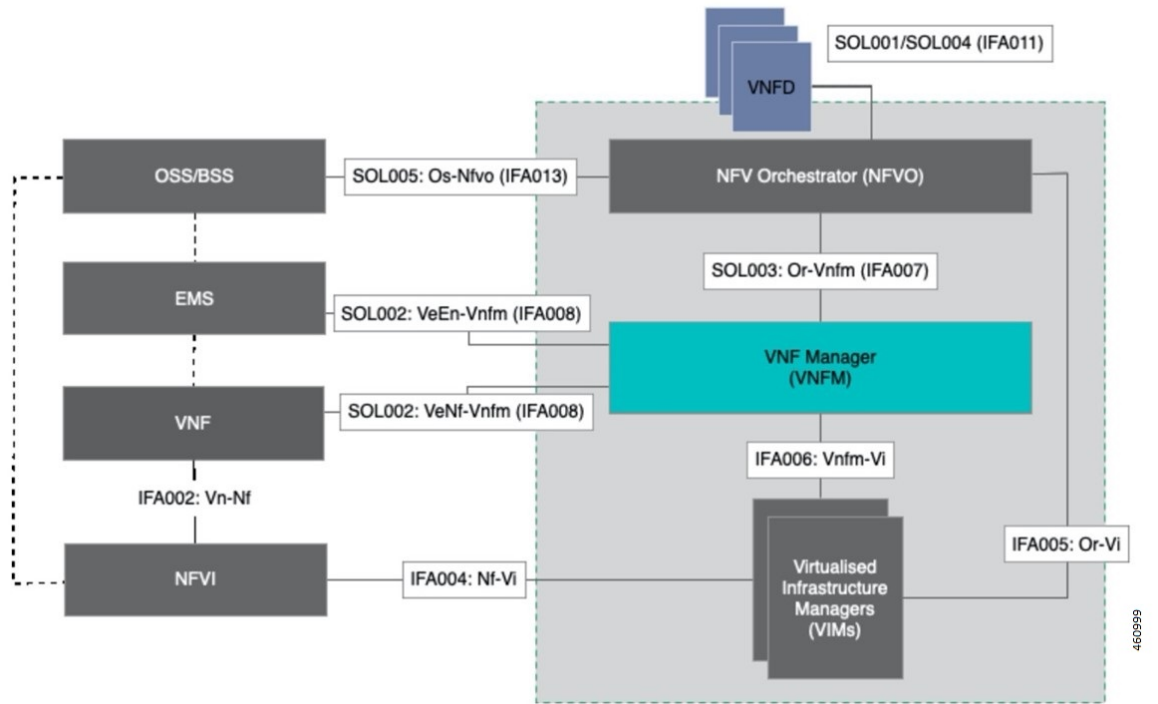
Figure 33: NFV Solution Architecture
