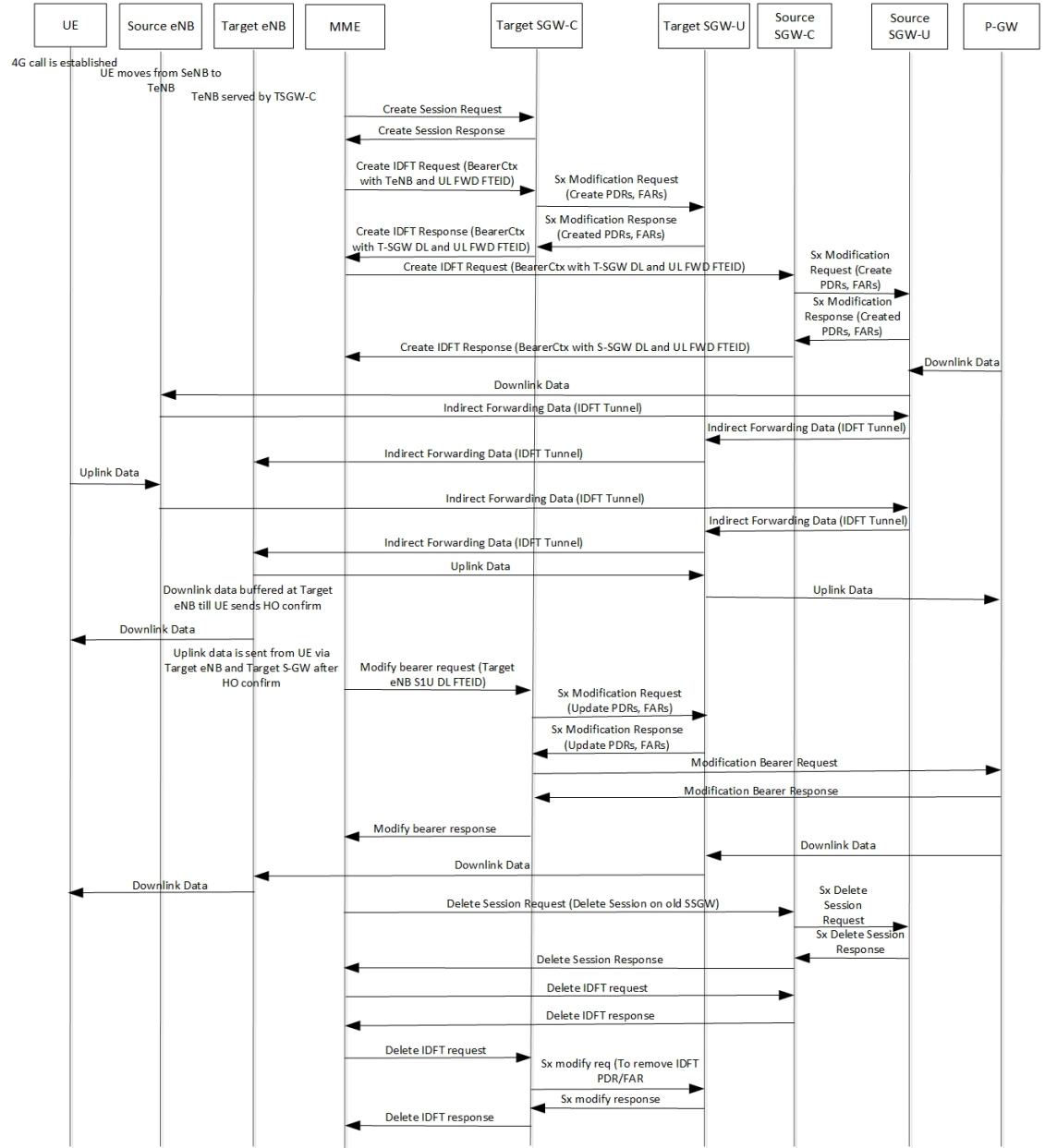
Figure 16: IDFT Support with S-GW Relocation
