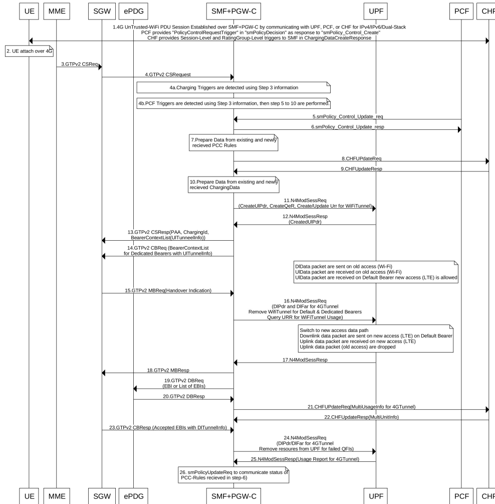
Figure 17: Non-3GPP Untrusted Wi-Fi to EPC Handover Call Flow
