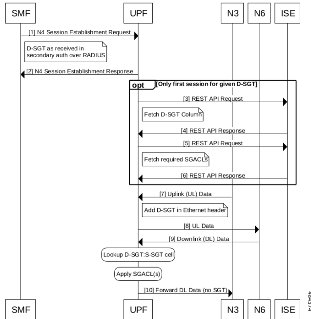
Figure 32: SGT Fetch and SGACL Enforcement Call Flow
