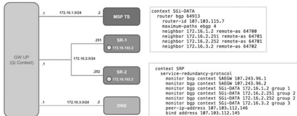
Figure 7: BGP Peer Groups and Routing
