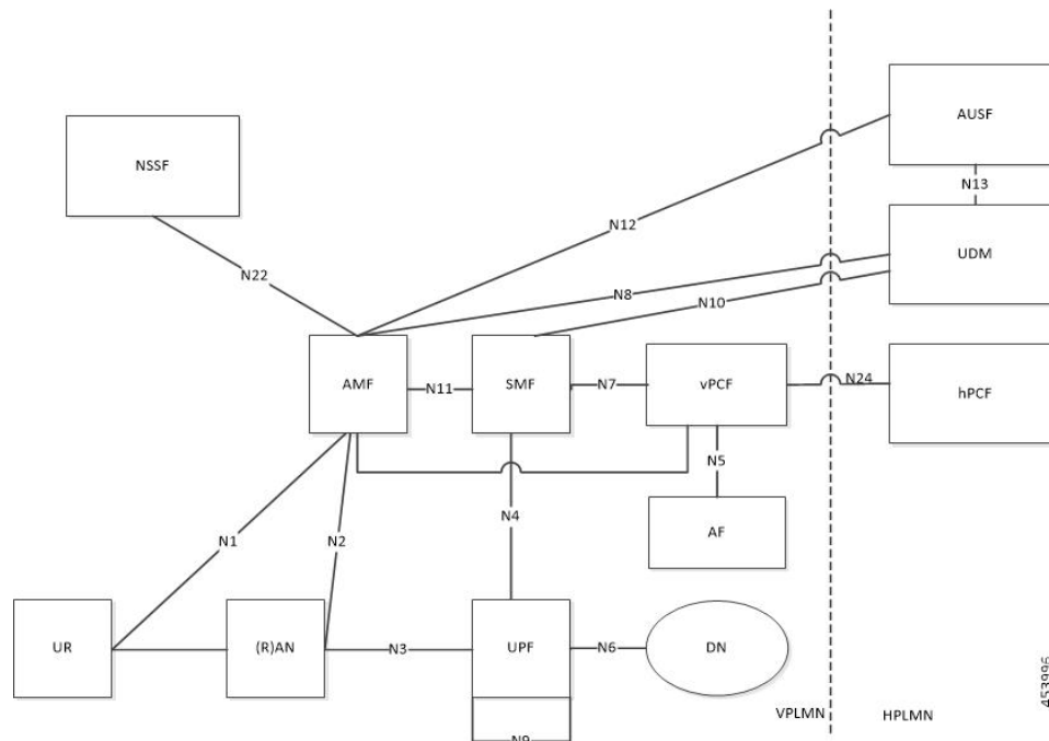
Figure 246: LBO Roaming Architecture for 5G Sessions
