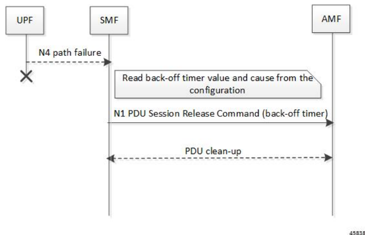
Figure 268: N4 Path Failure Handling Call Flow for Non-roaming Session
