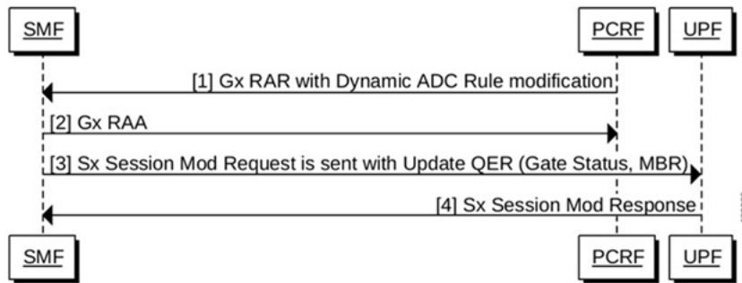
Figure 217: Dynamic ADC Rule Modification Call Flow
