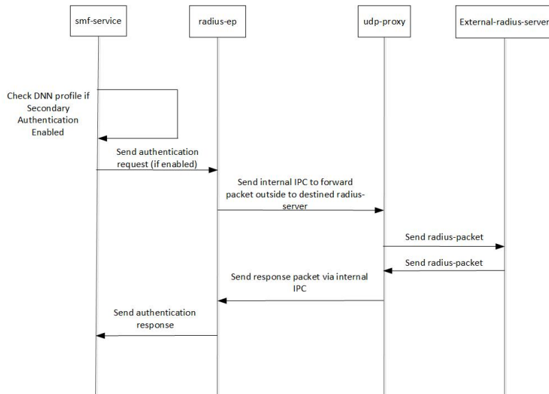
Figure 234: RADIUS Authentication Call Flow
