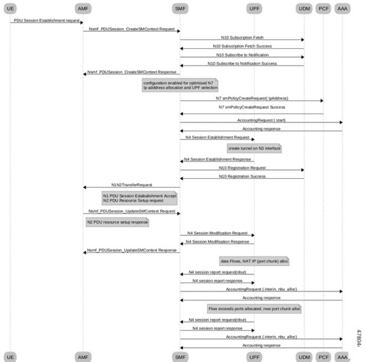
Figure 174: Call Flow for Port Chunk Allocation
