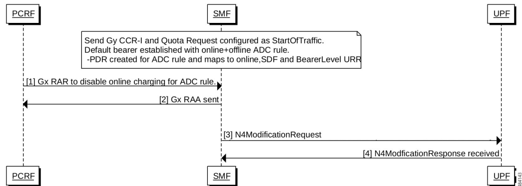
Figure 218: Call Flow for Charging Modification from Both Offline and Online to Offline Only
