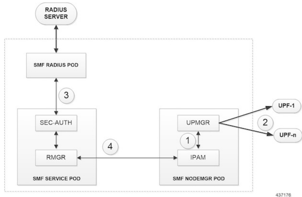
Figure 172: Static IP Address Management Procedure
