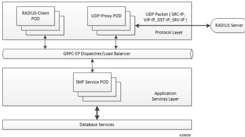
Figure 233: RADIUS Client Integration
