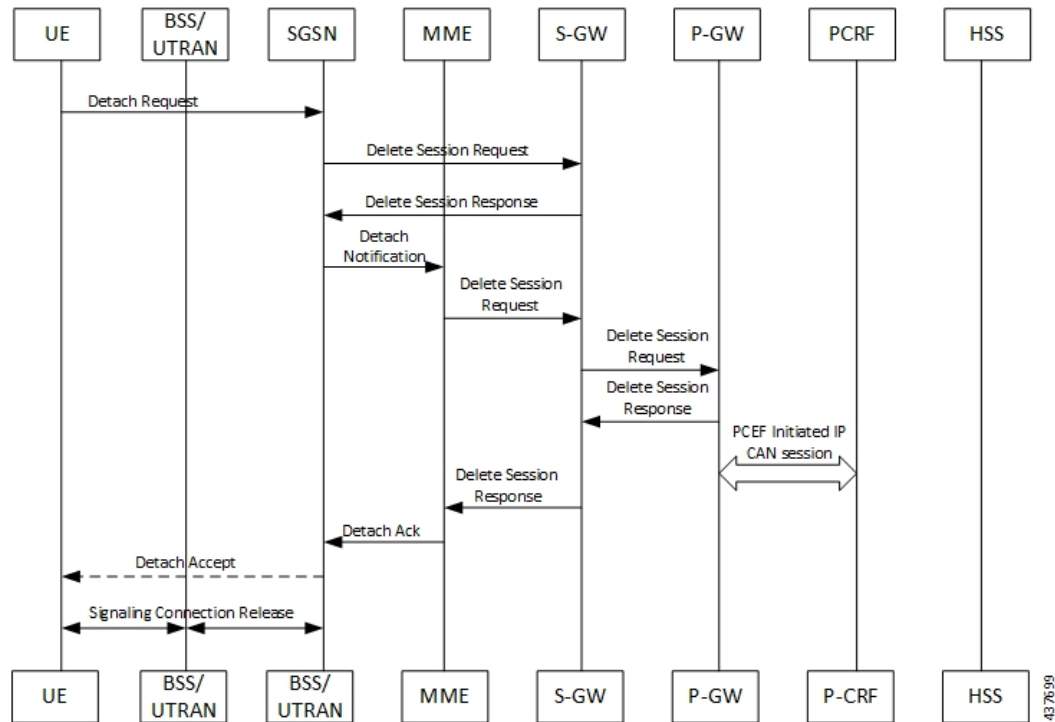
Figure 32: UE-initiated EPS Call Release Flow
