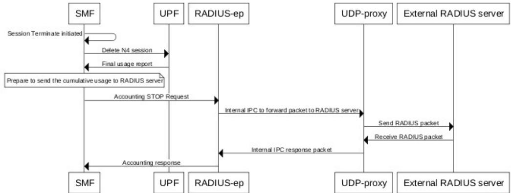
Figure 236: RADIUS Accounting Stop Call Flow
