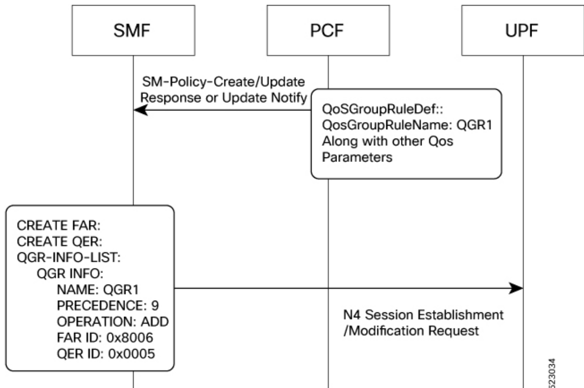
Figure 230: Qos-Group-of-Ruledef Activation Call Flow
