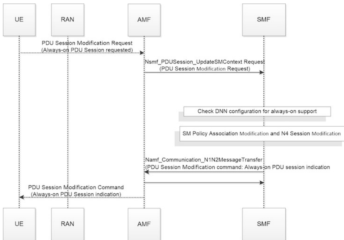
Figure 288: UE-requested PDU Session Modification Call Flow
