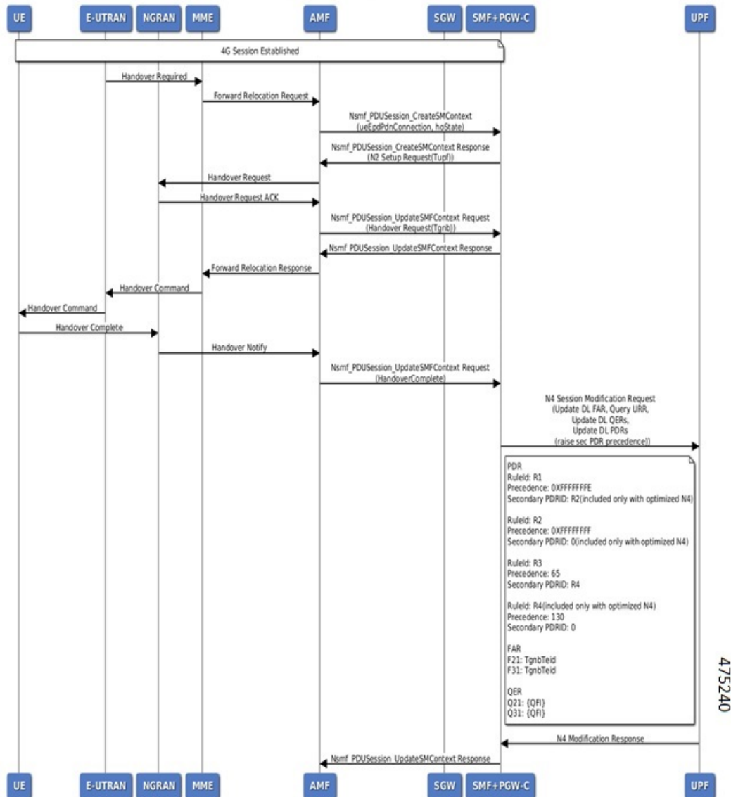
Figure 267: Call Flow for Inter-plmn HO from 4G Roamer to 5G Homer
