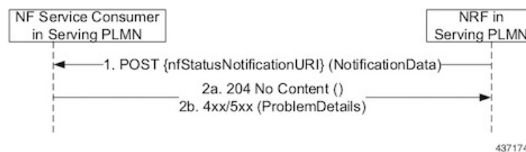
Figure 197: NFStatus Notify Call Flow
