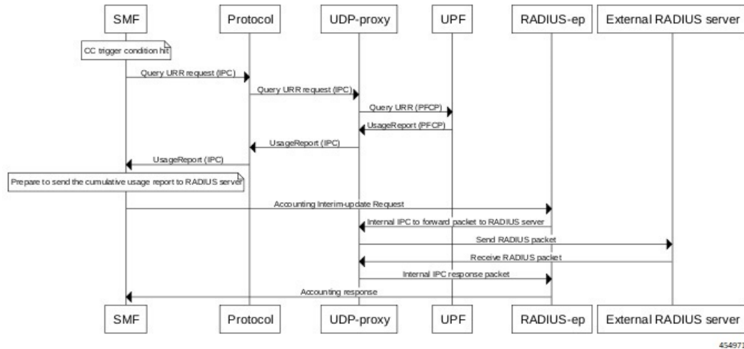
Figure 238: Synchronous Accounting Interim-Update Call Flow
