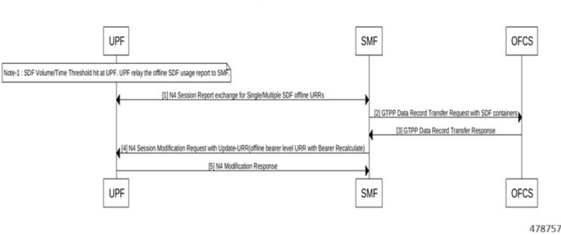
Figure 144: Call Flow for Asynchronous Usage report for offline Bearer recalculatio
