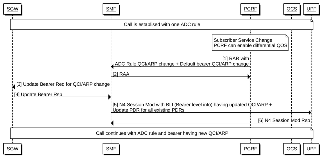
Figure 220: Call Flow for Modifying QCI and ARP of an Installed Dynamic ADC Rule
