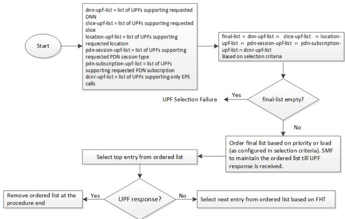
Figure 222: UPF Node Selection Workflow
