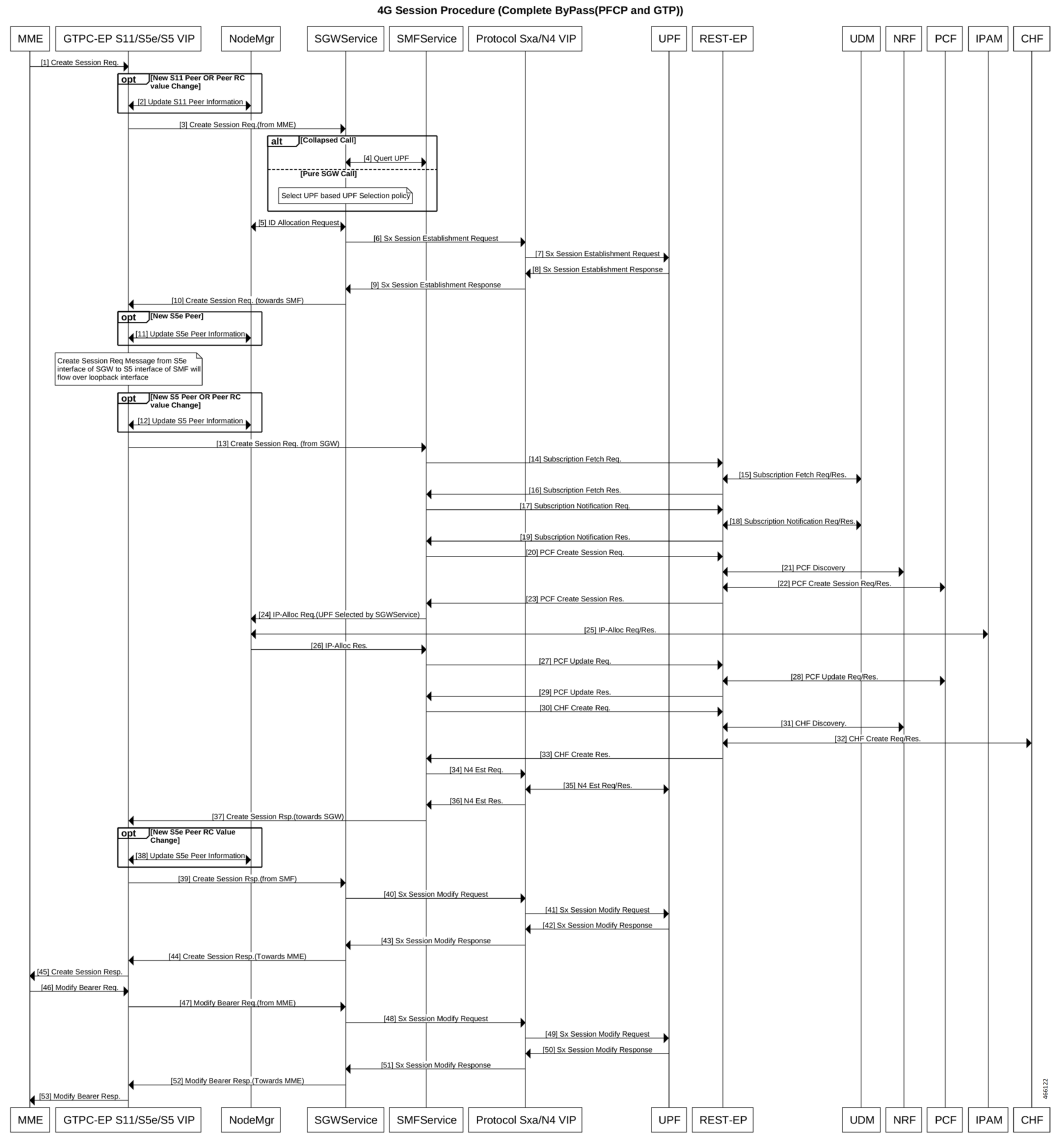
Figure 8: 4G Session Procedure - Complete Bypass(PCFP and GTP)
