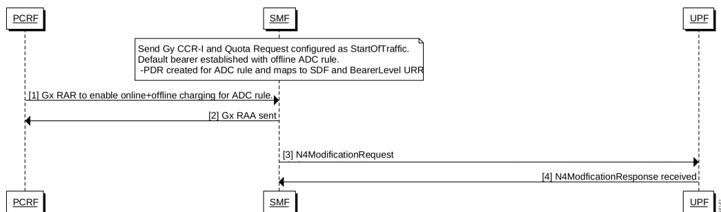
Figure 219: Call Flow for Charging Modification from Offline Only to Both Offline and Online
