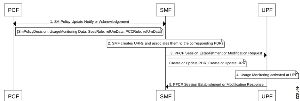
Figure 223: Usage Monitoring Activation Call Flow
