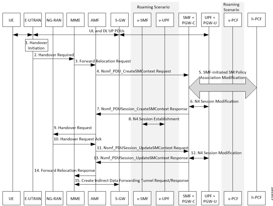
Figure 256: Call Flow for the EPS to 5G Handover Using the N26 Interface
