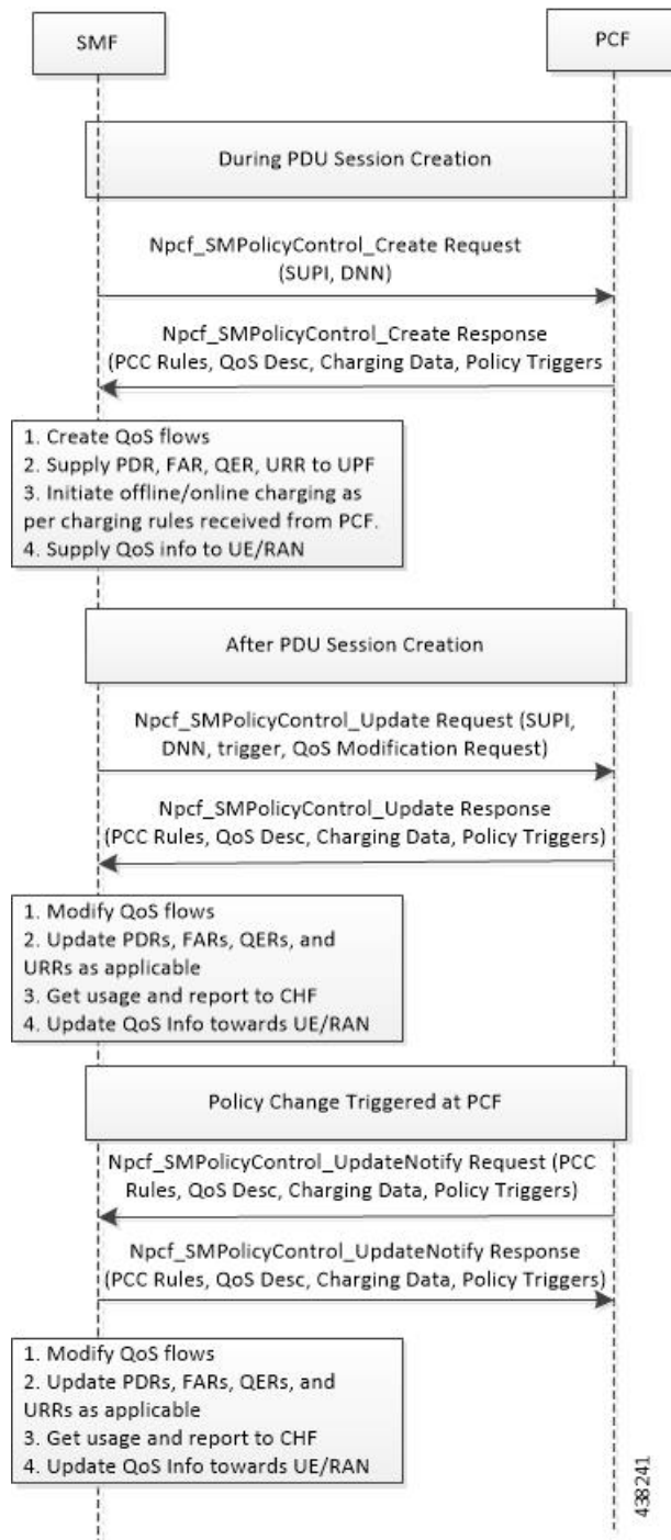
Figure 213: Dynamic Policy Management Call Flow
