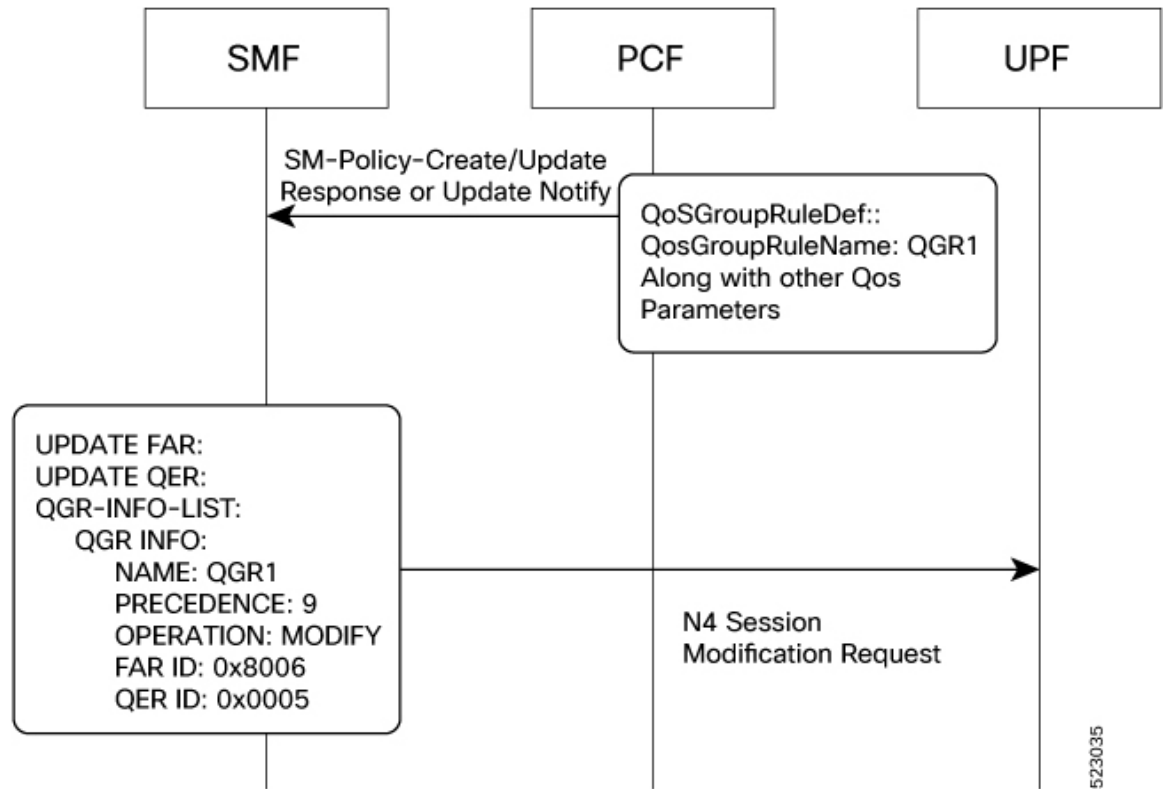
Figure 231: Qos-Group-of-Ruledef Modification Call Flow
