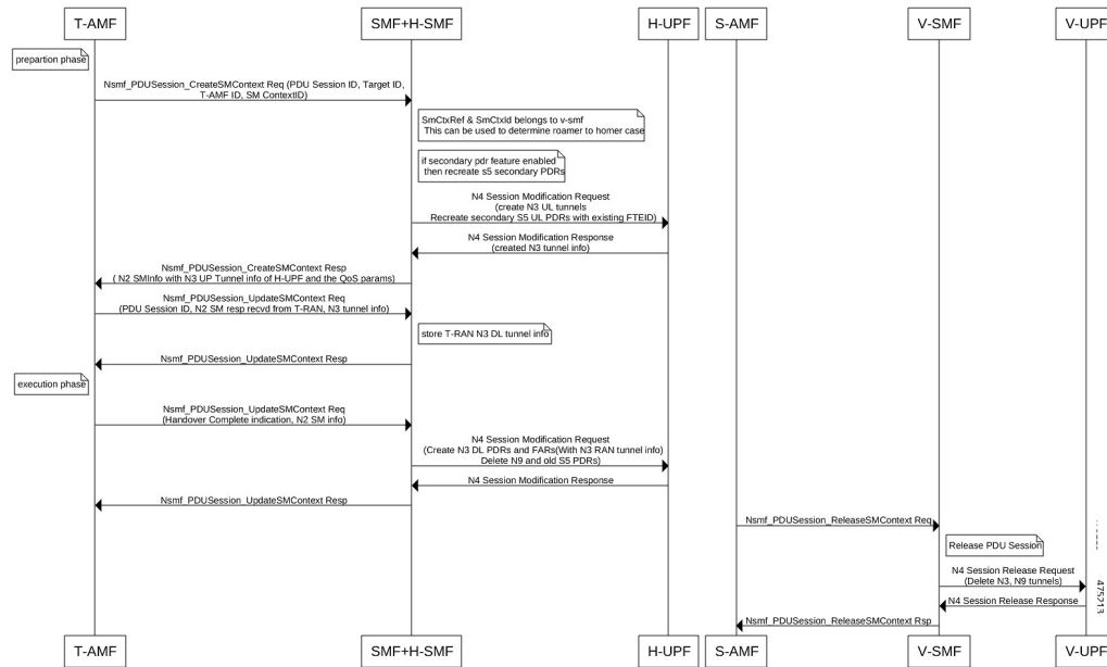
Figure 262: Call Flow for Inter-plmn N2 HO with v-SMF Deletion
