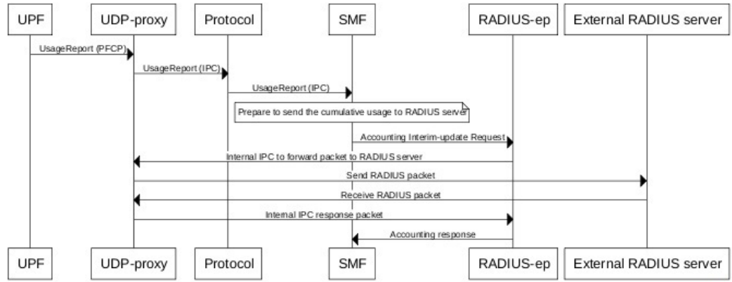
Figure 237: Asynchronous Accounting Interim-Update Call Flow
