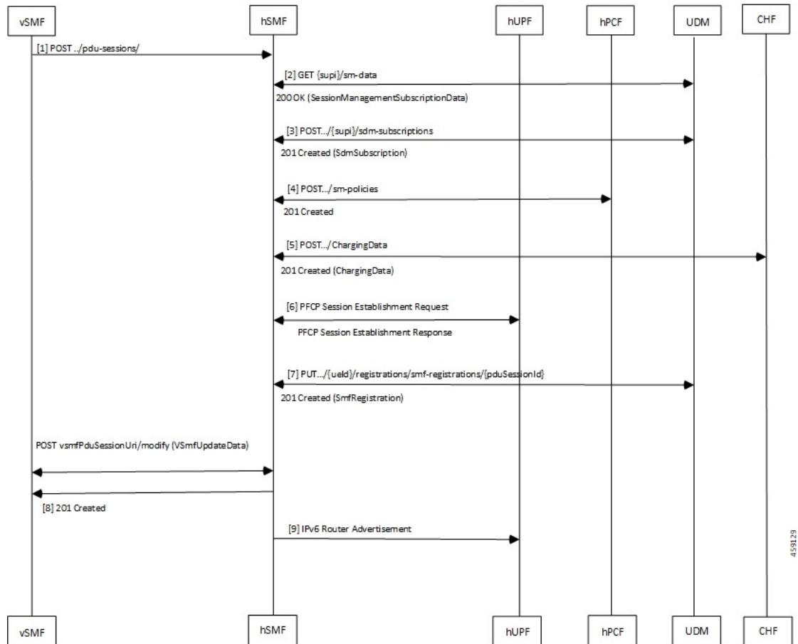
Figure 250: hSMF Create Session Call Flow
