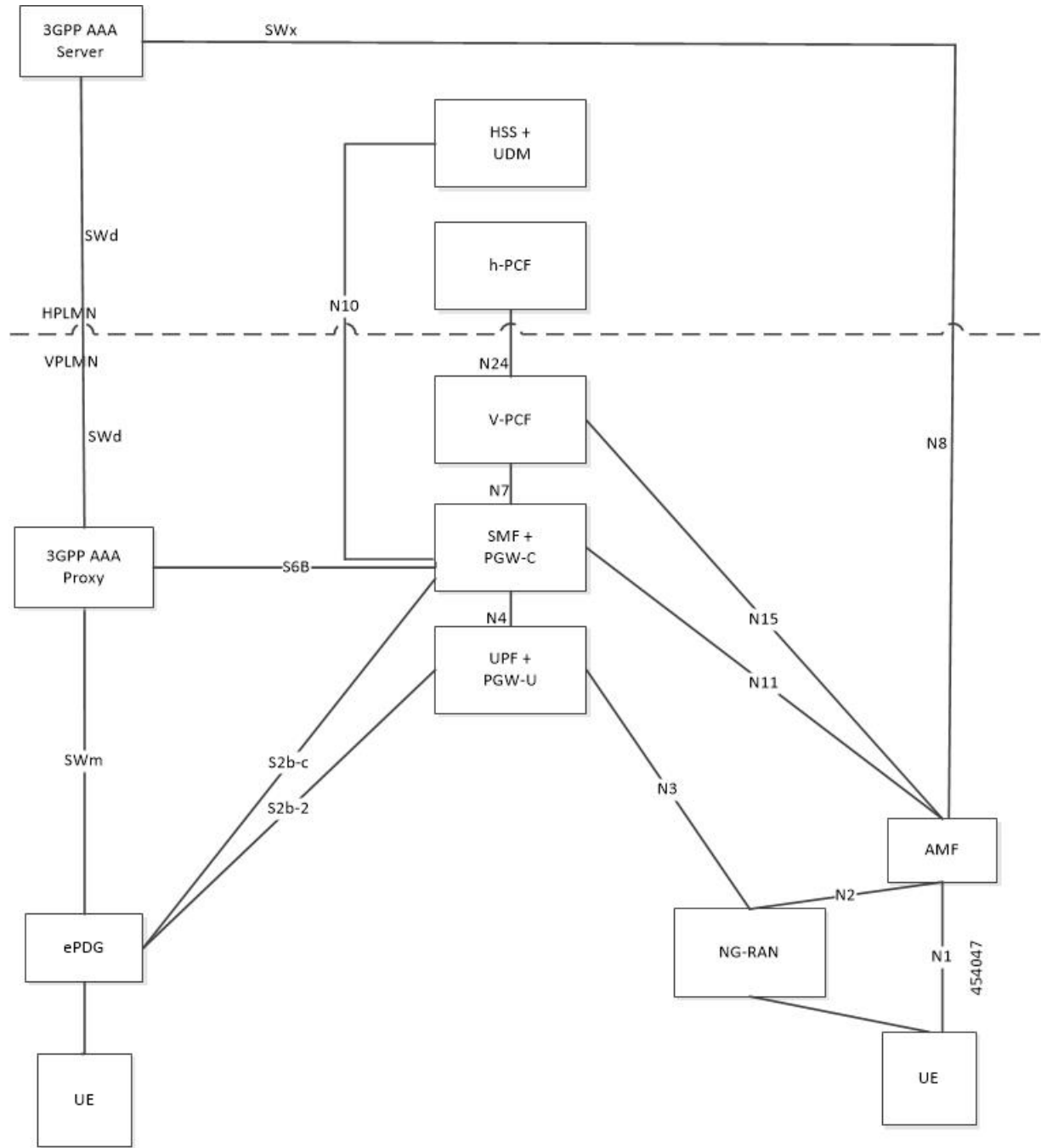
Figure 245: Local Breakout Roaming Architecture for Wi-Fi Sessions
