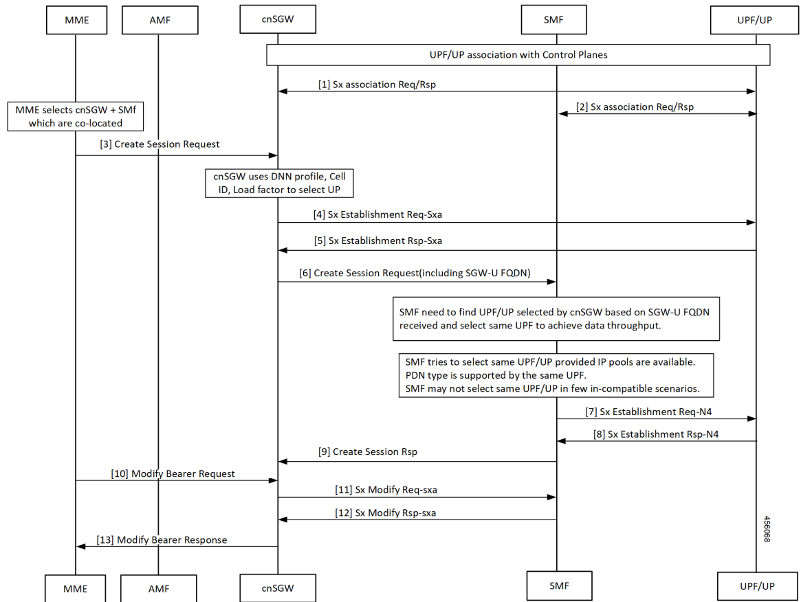
Figure 133: Initial Attach on 4G for 5G Capable Device Call Flow
