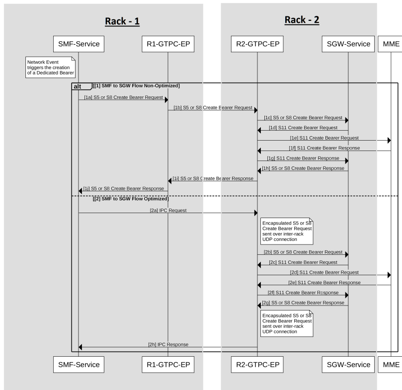
Figure 105: SMF and PGWc GTPC Optimization with Inter-rack IPC Call Flow
