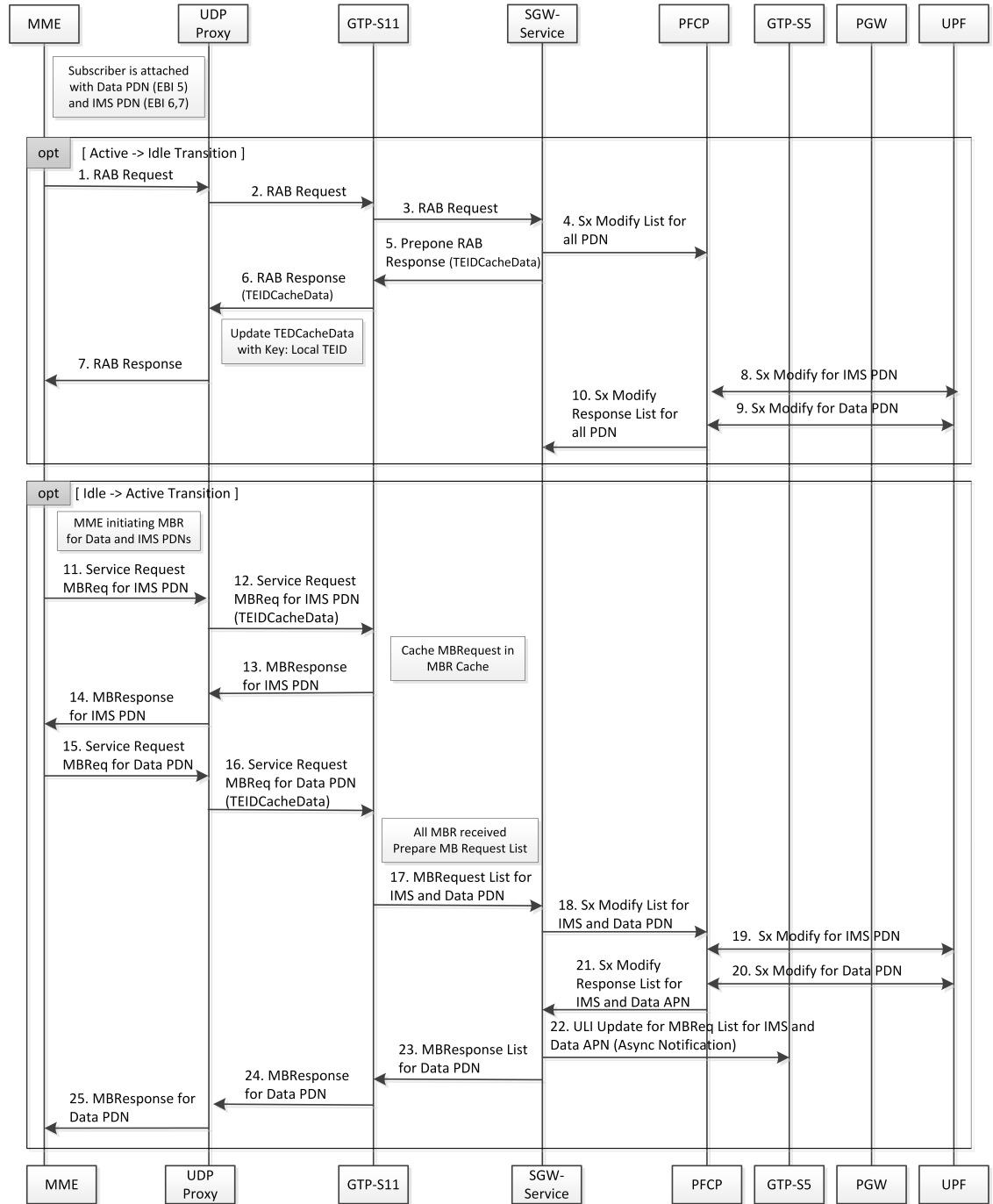
Figure 108: MBR Optimization Call Flow
