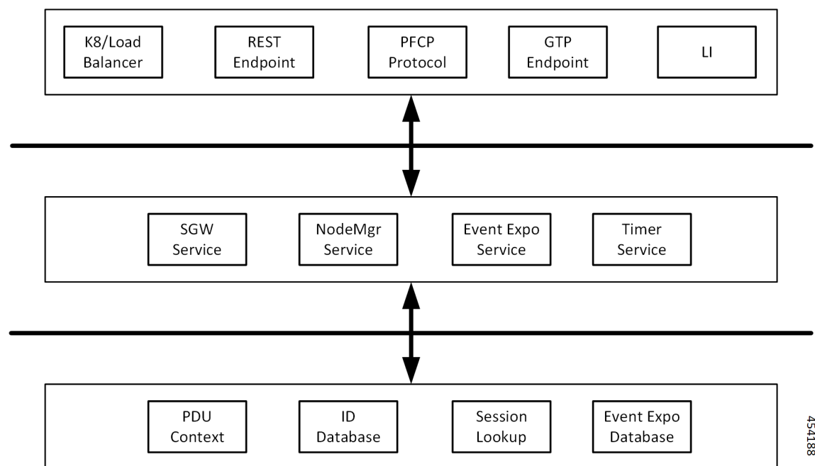
Figure 5: cnSGW-C Architecture
