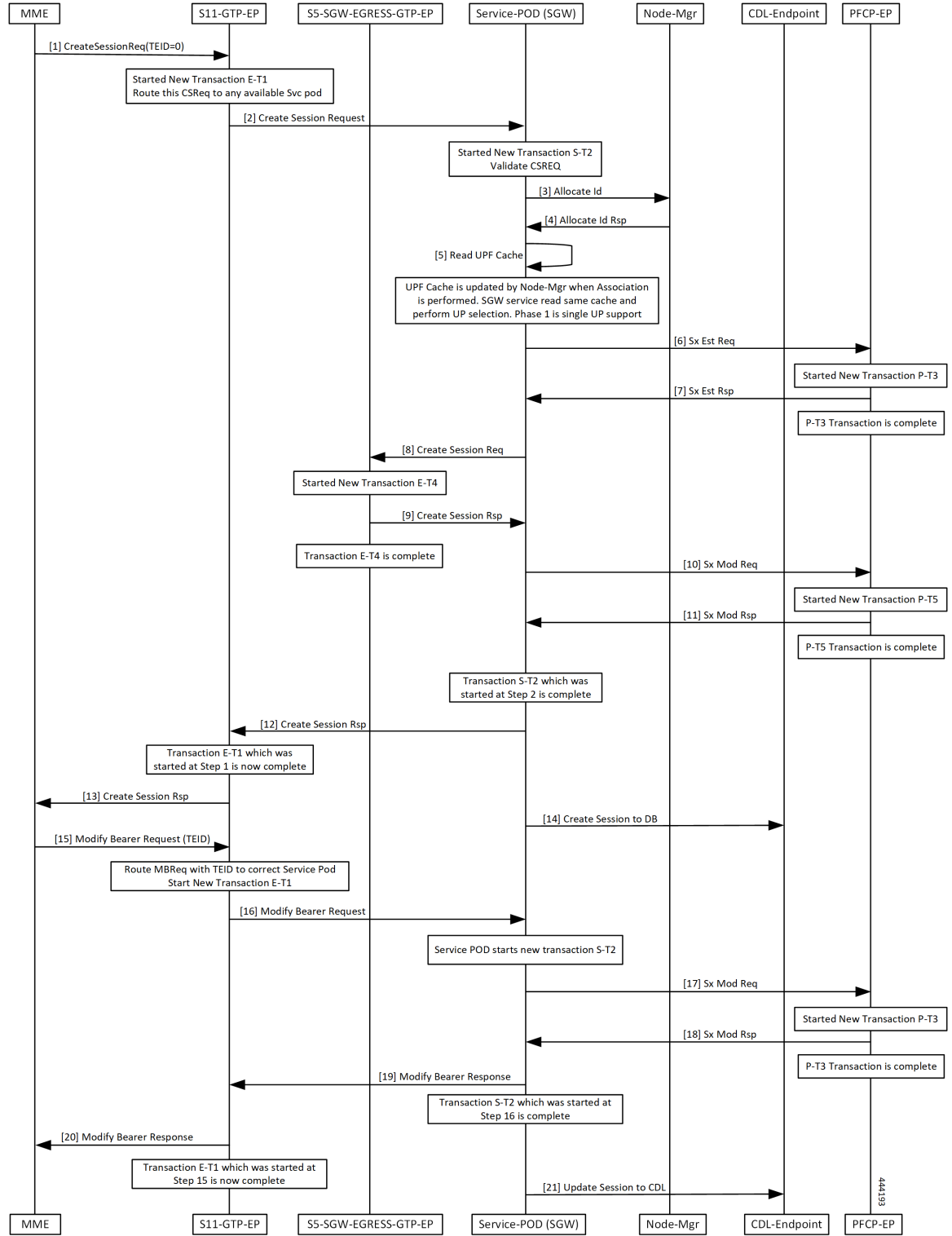
Figure 69: Initial Attach Call Flow
