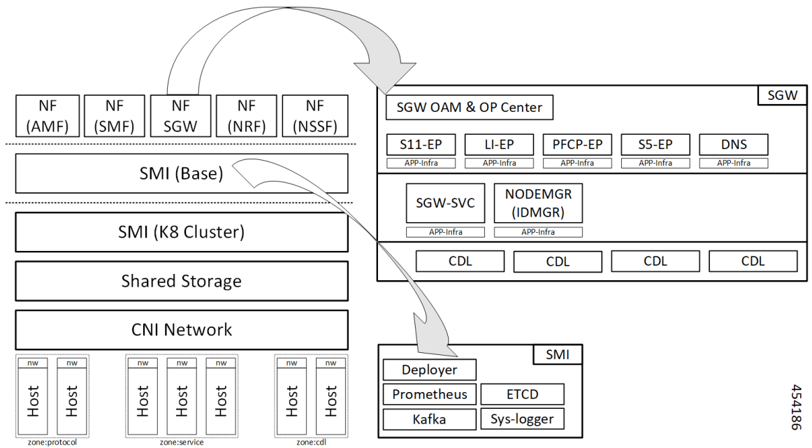
Figure 6: cnSGW-C Deployment
