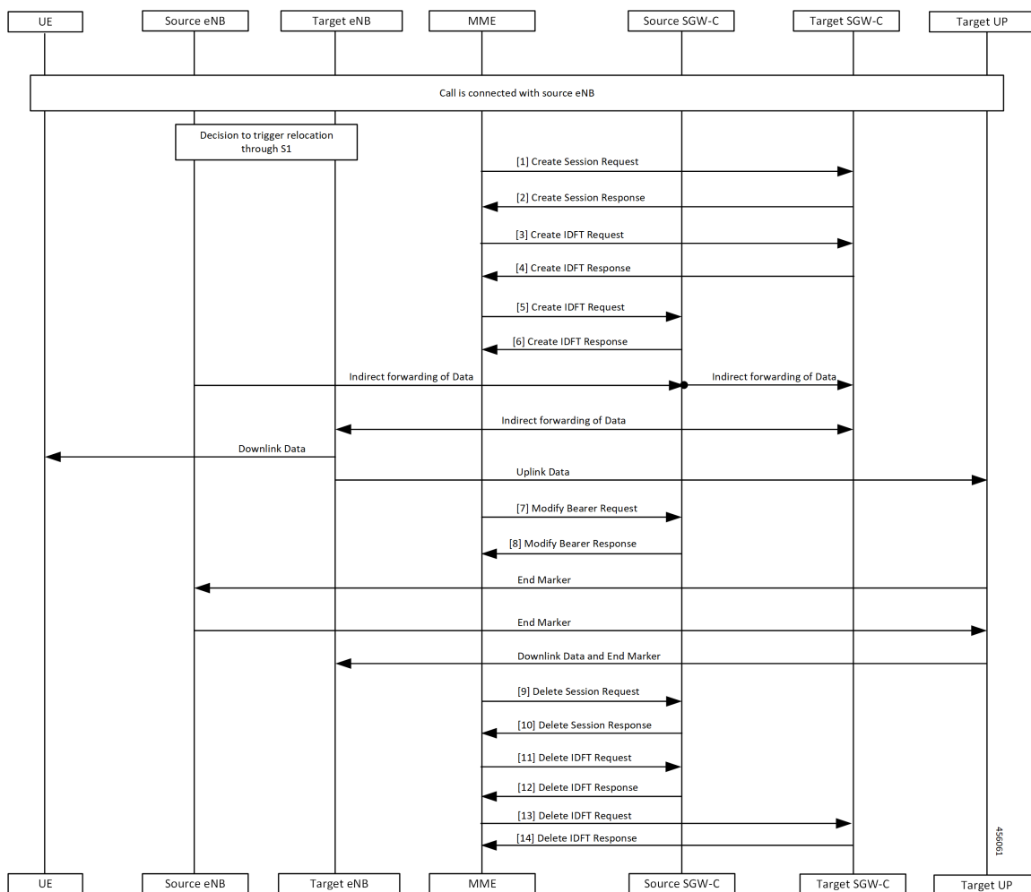
Figure 60: IDFT Support with SGW Relocation Call Flow
