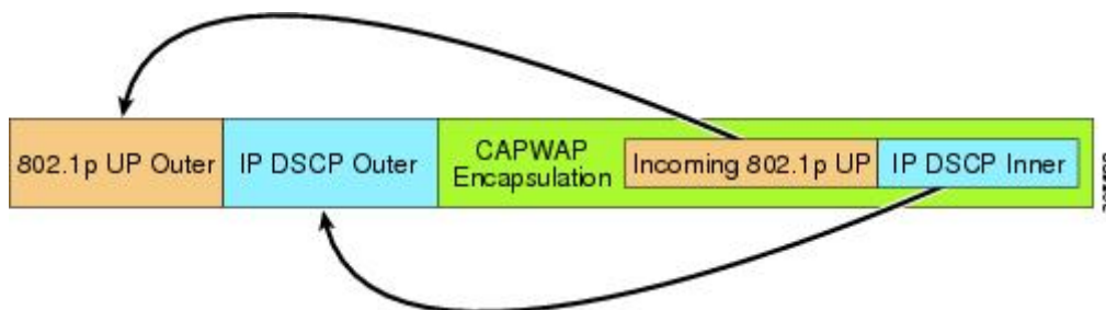
Figure 48: Controller to RAP Path
