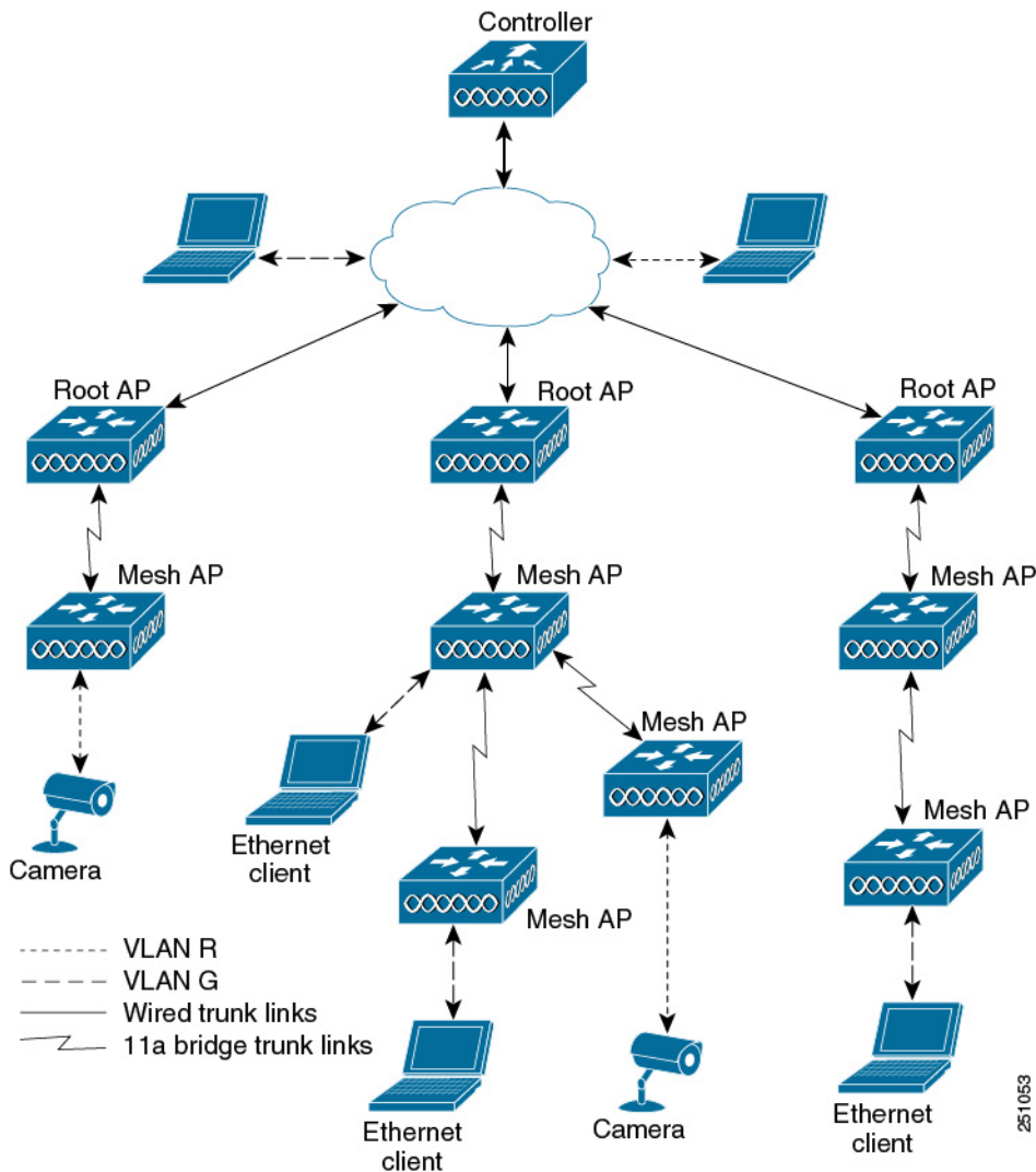
Figure 35: Ethernet VLAN Tagging
