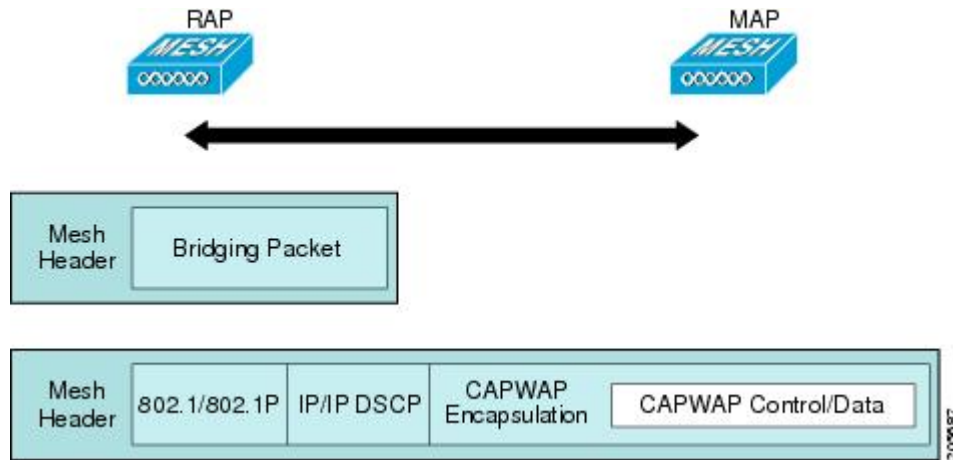
Figure 47: Encapsulating Mesh Traffic
