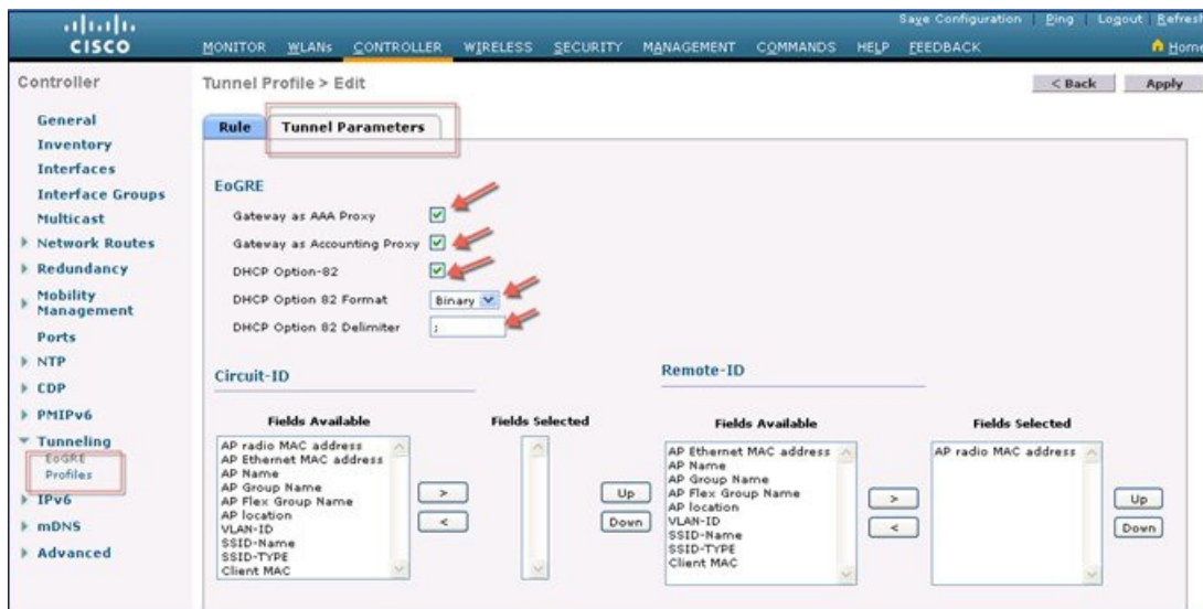
Figure 1: DHCP Option-82 Configuration From the GUI Interface
