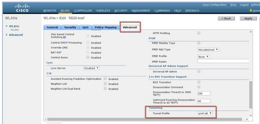
Figure 3: Mapping the profile "prof-att" to WLAN
