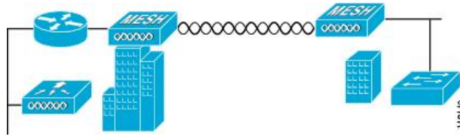
Figure 2: Point-to-Point Bridging Example
