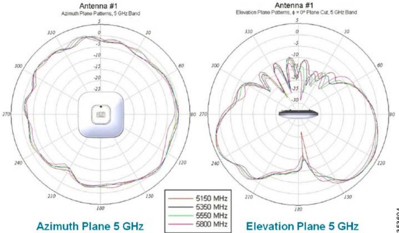
Figure 104 Patterns Azimuth and Elevation Plane @ 5 GHz
