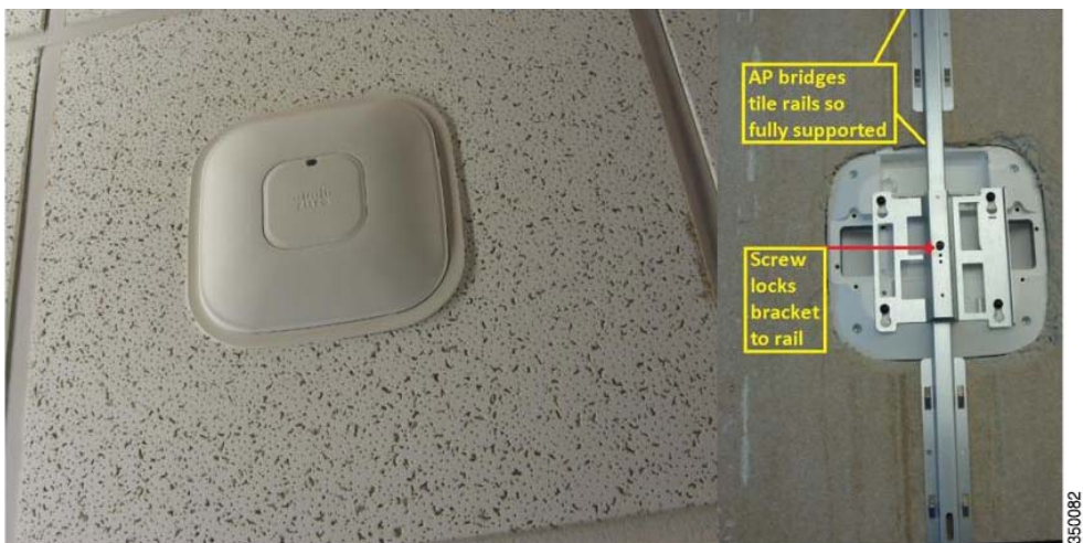
Figure 16 Optional AIR-AP-BRACKET-3 Used to Install the AP Directly Into the Tile
