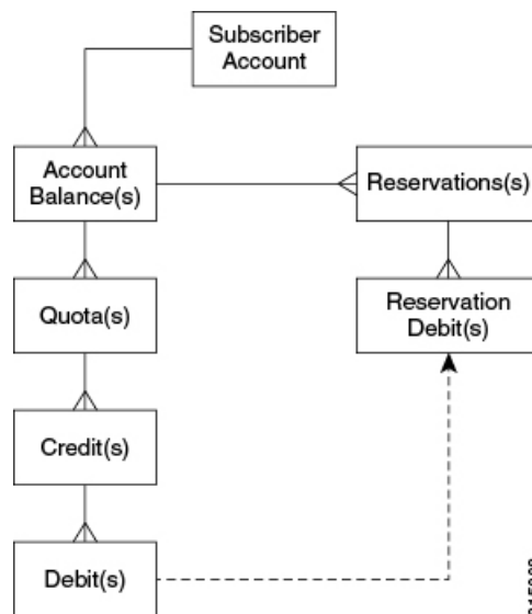
Figure 6: Subscriber Records
