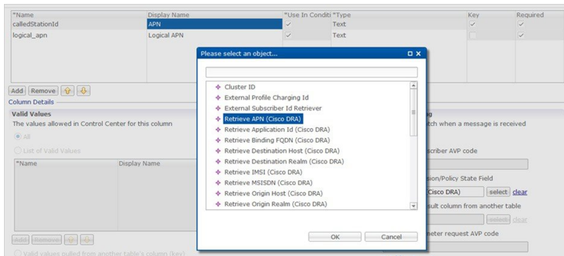
Figure 72: Adding AVPs
