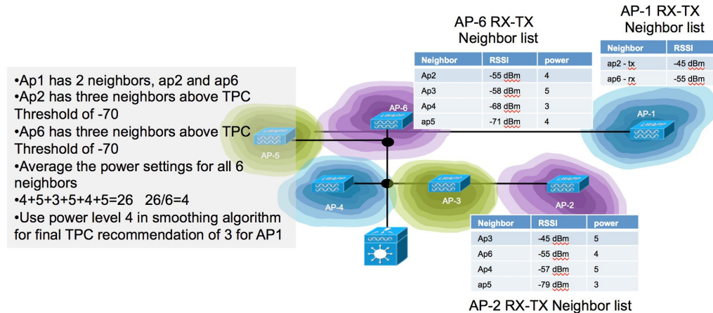
Figure 24: TPCv1 Smoothing Algorithm function
