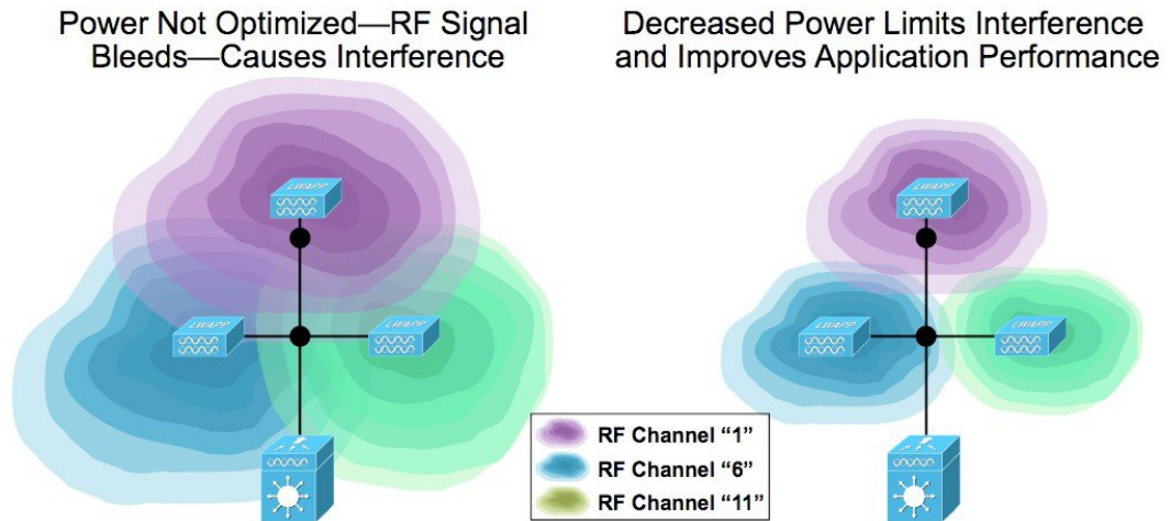
Figure 23: TPC Maximizes Coverage, Minimizes CCI
