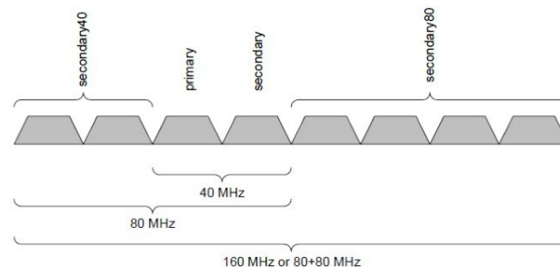
Figure 15: OBSS Channel Architecture
