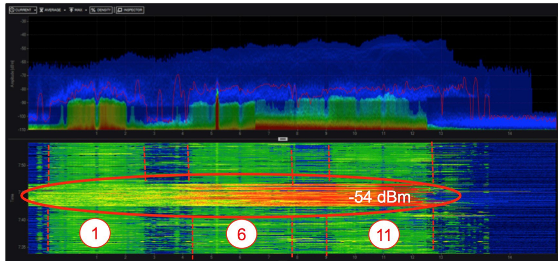
Figure 20: Microwave Oven impact - Channelizer Pro
