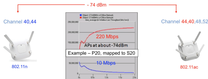
Figure 16: Destructive Coexistence Example
