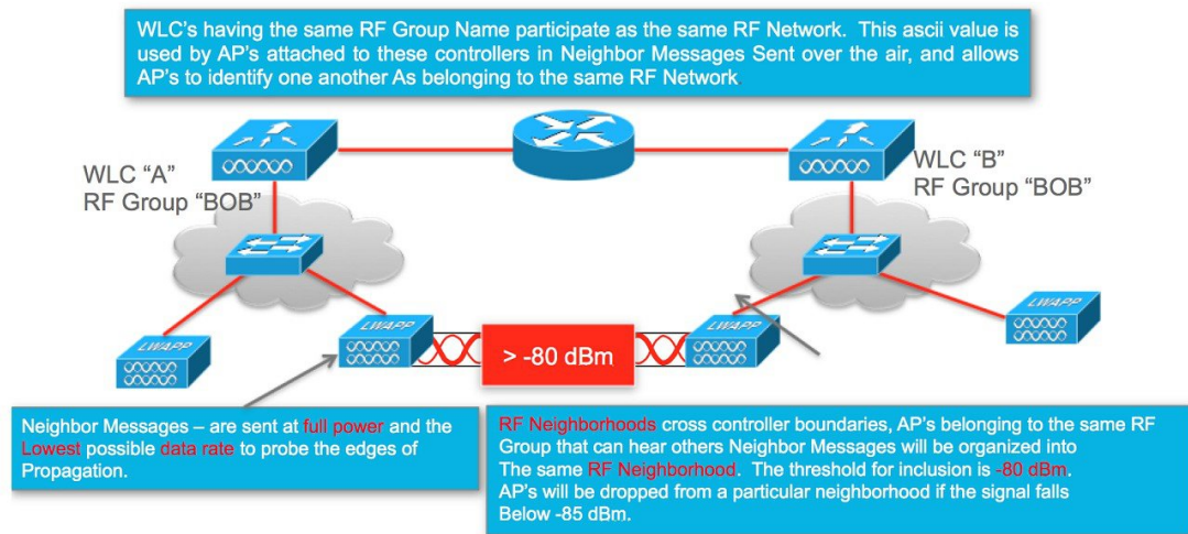
Figure 6: RF Group and Neighborhood example
