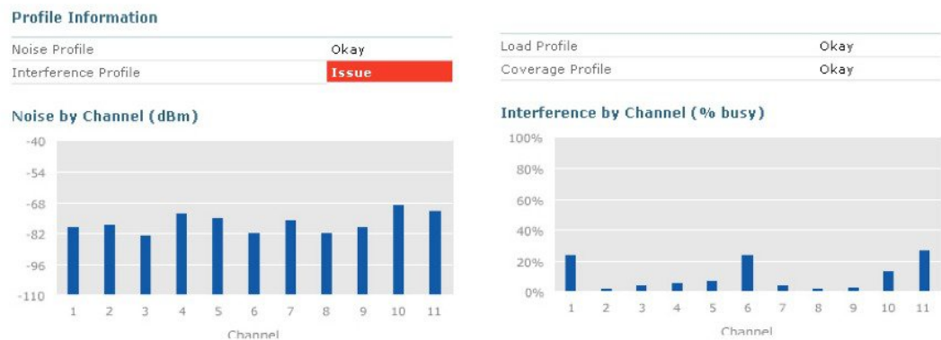
Figure 12: View of Interference and Noise from the Radio Page on a Controller
