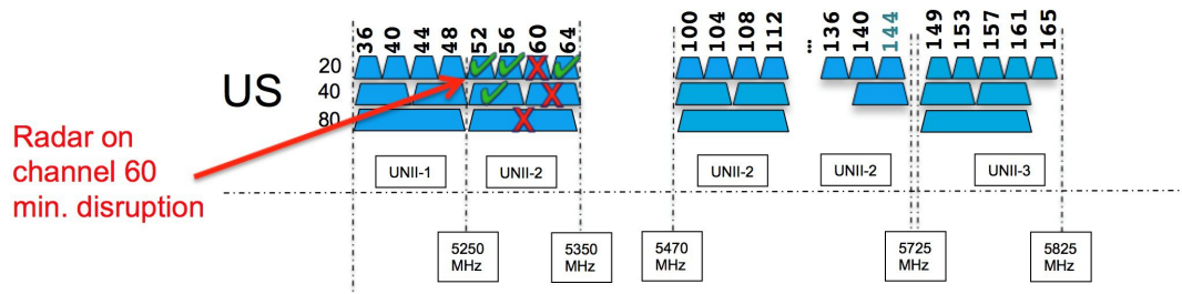
Figure 19: Example of Flex DFS channel options
