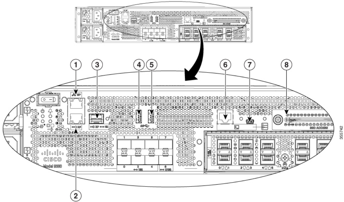
Figure 3: Management and Storage Connections for the Cisco Catalyst 9800-80 Wireless Controller
