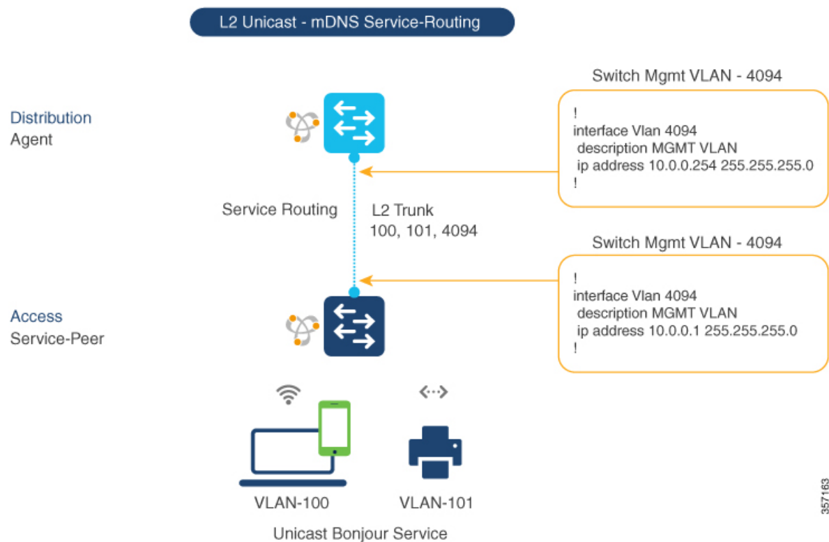
Figure 73: Catalyst Service-Peer Service-Routing Configuration
