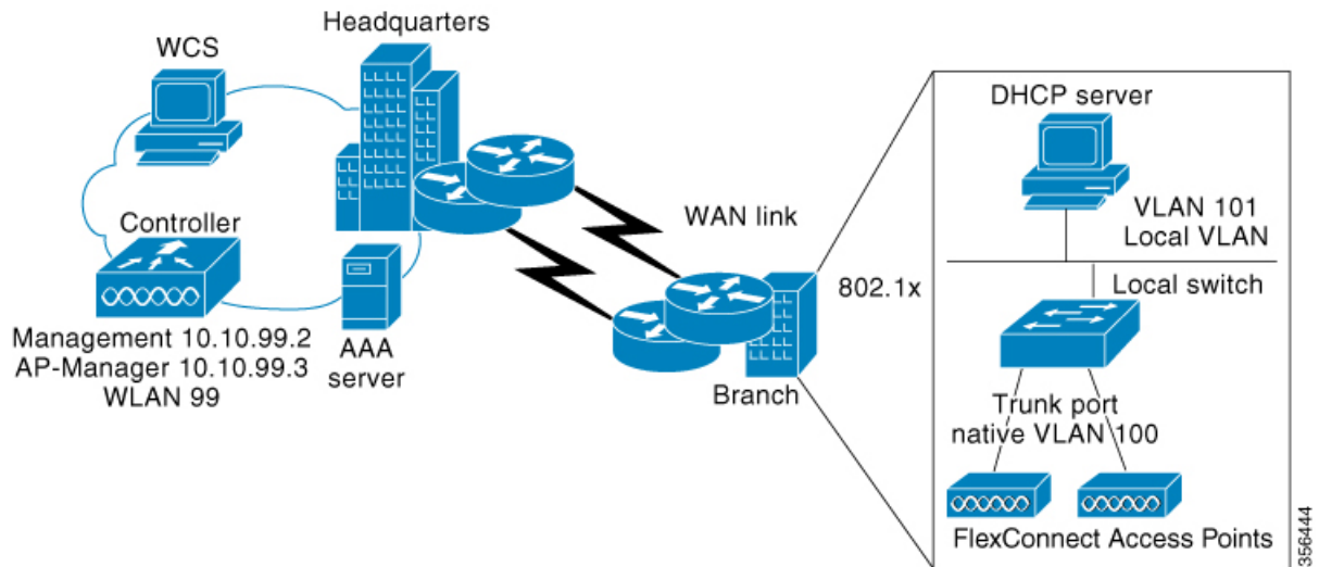
Figure 16: FlexConnect Deployment
