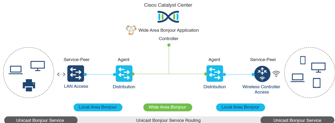
Figure 54: Cisco Wide Area Bonjour Solution Architecture
