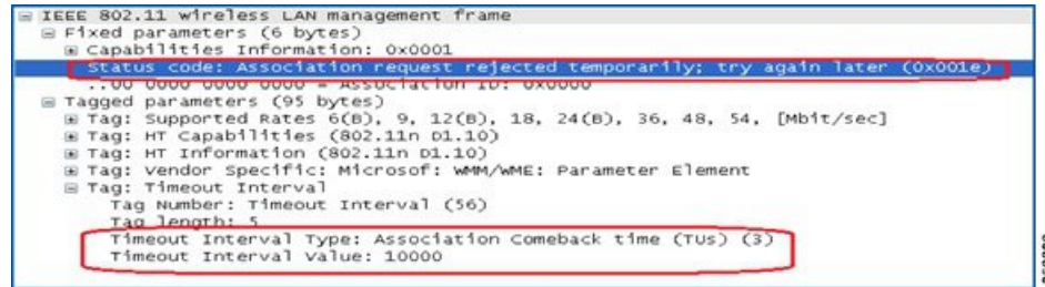
Figure 32: Association Reject with Comeback Time
