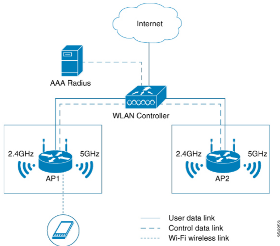
Figure 19: Wi-Fi Agile Multiband Wireless Infrastructure Network
