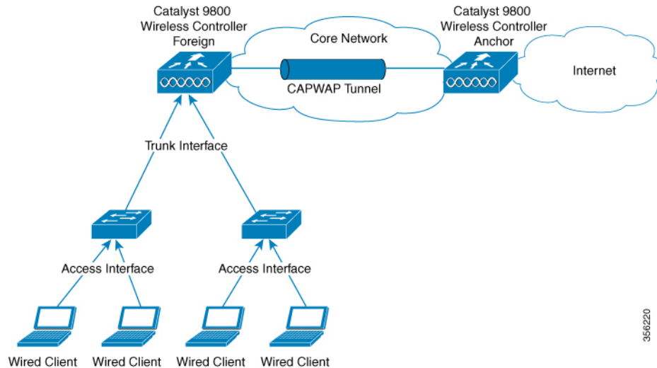
Figure 48: Guest Access Architecture
