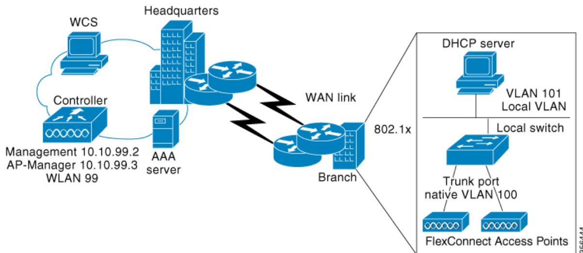
Figure 13: FlexConnect Deployment
