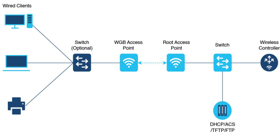
Figure 41: Example of a WGB
