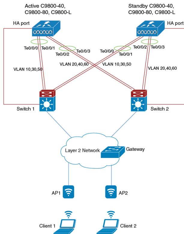
Figure 50: SSO Pair with Multi-LAG
