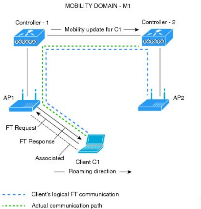
Figure 44: Message Exchanges when Over-the-DS Client Roaming is Configured
