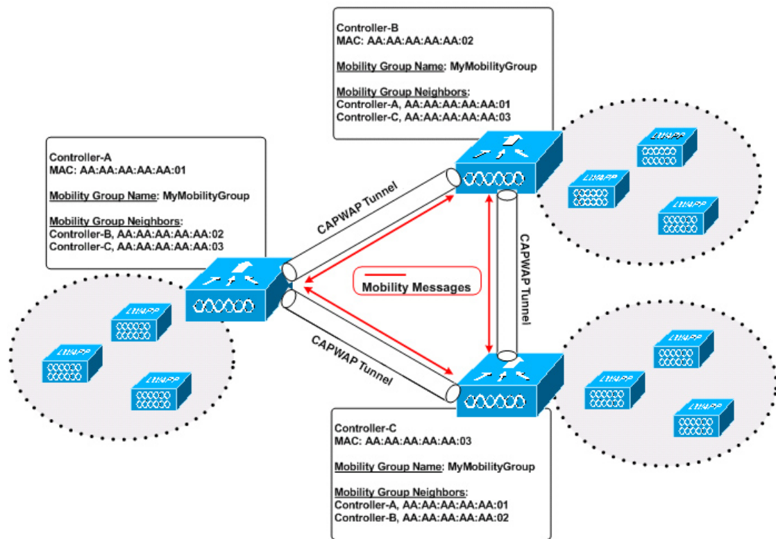
Figure 33: Example of a Single Mobility Group
