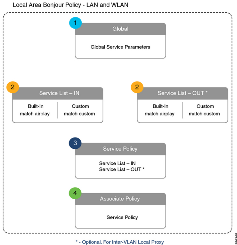
Figure 17: Local Area Bonjour Policy Hierarchy
