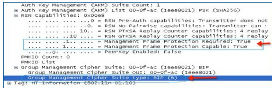
Figure 47: 802.11w Information Elements
