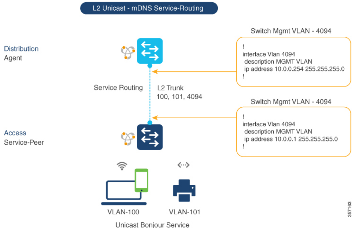
Figure 68: Catalyst Service-Peer Service-Routing Configuration
