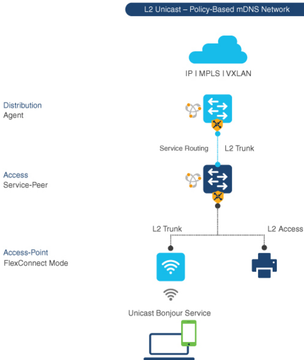
Figure 66: mDNS Service Policy Configuration on Catalyst Switch in Service-Peer and SDG Agent Modes
