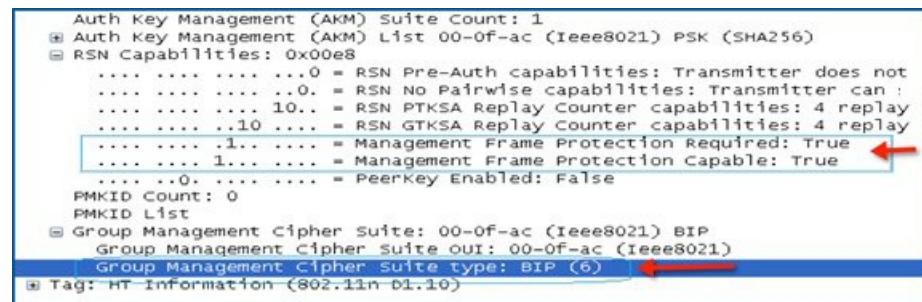
Figure 46: 802.11w Information Elements
