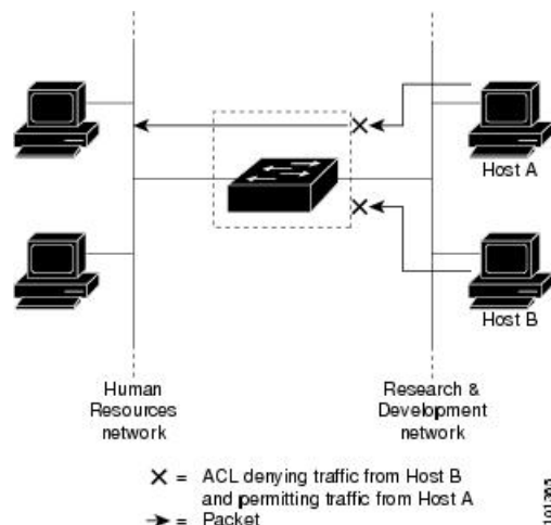
Figure 17: Using ACLs to Control Traffic in a Network
