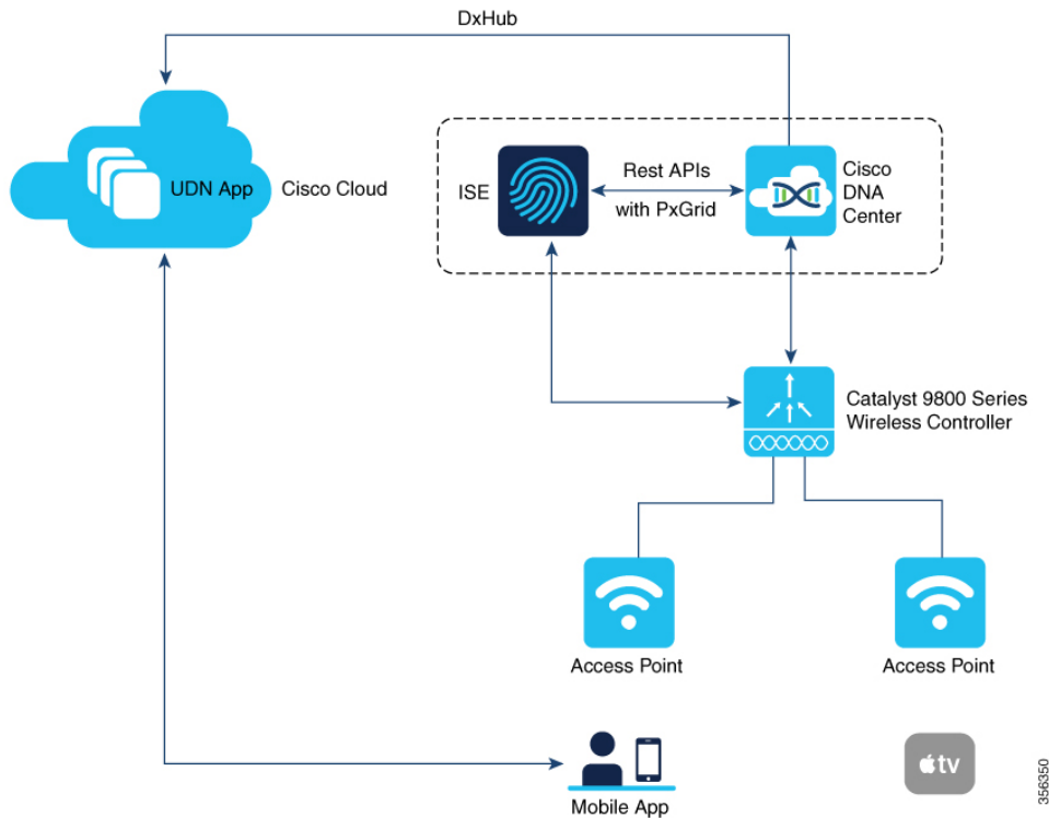
Figure 51: User Defined Network Topology
