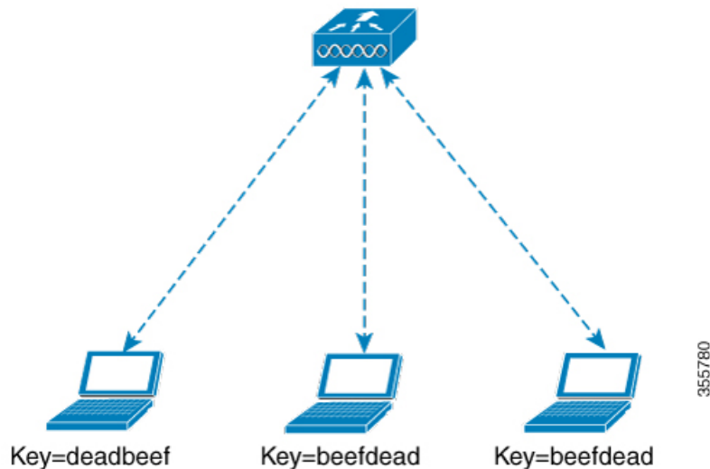
Figure 25: Multi-PSK
