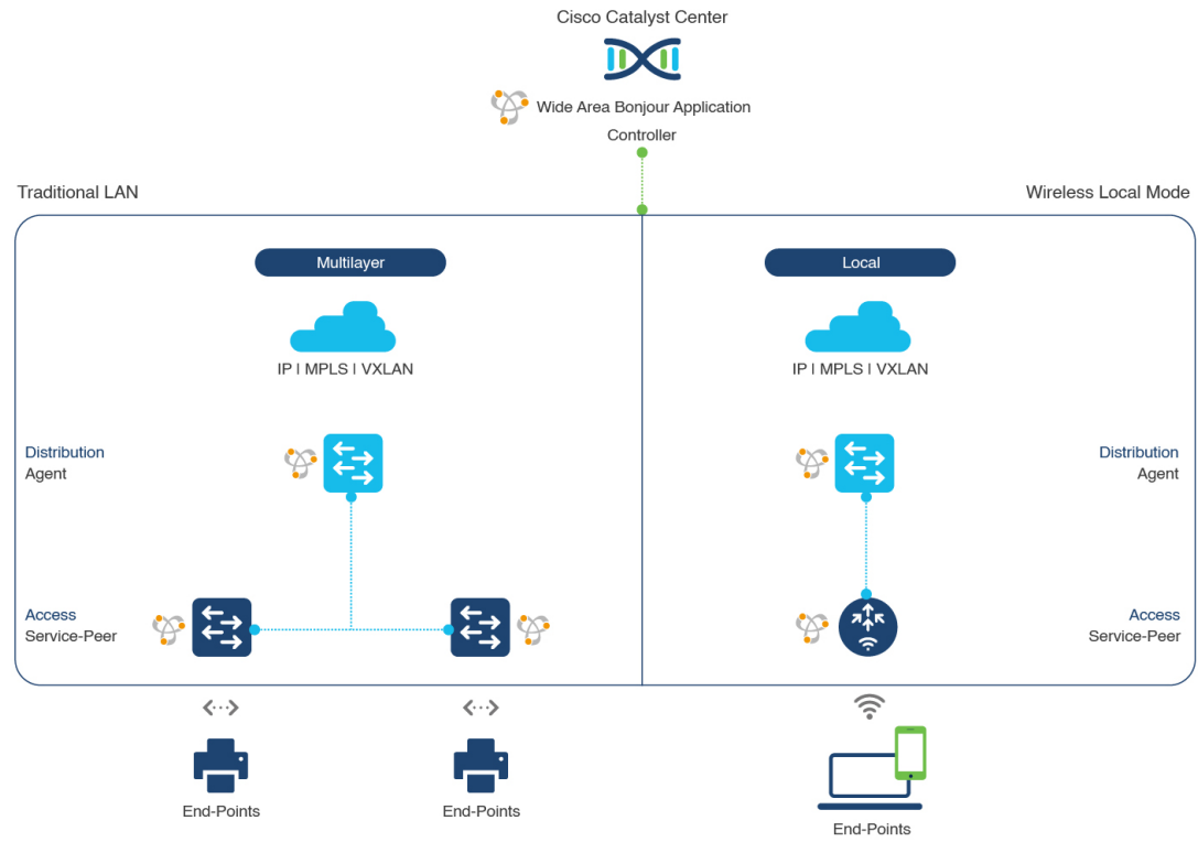
Figure 53: Enterprise Traditional LAN and Wireless Local Mode Network Design
