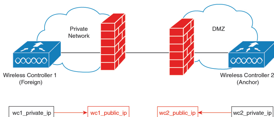
Figure 33: Mobility NAT
