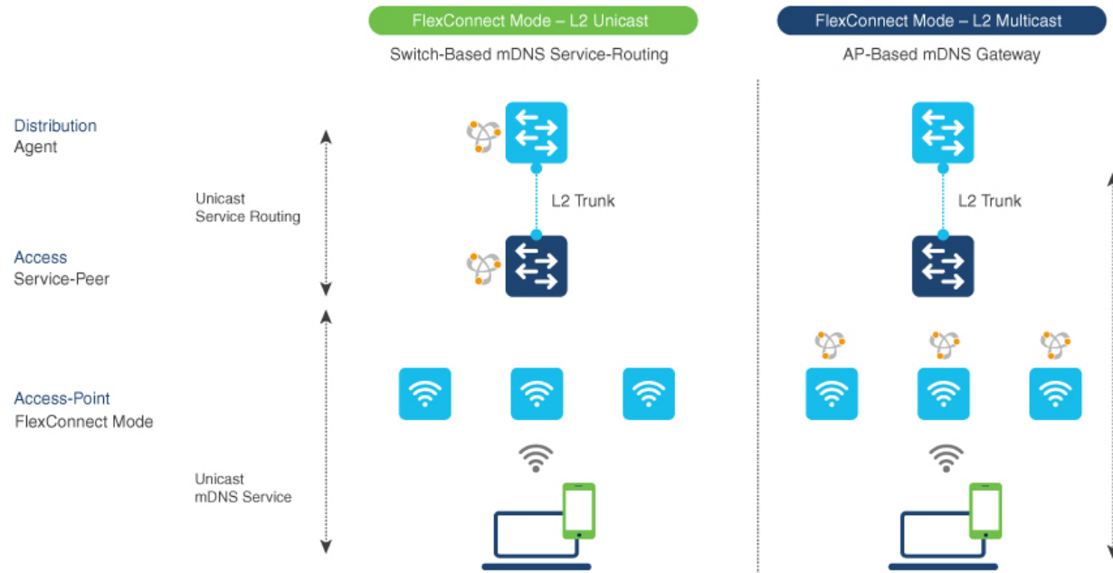
Figure 63: mDNS Gateway Alternatives for FlexConnect Mode
