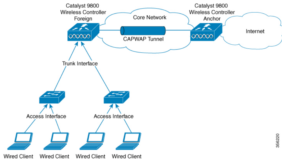
Figure 41: Guest Access Architecture
