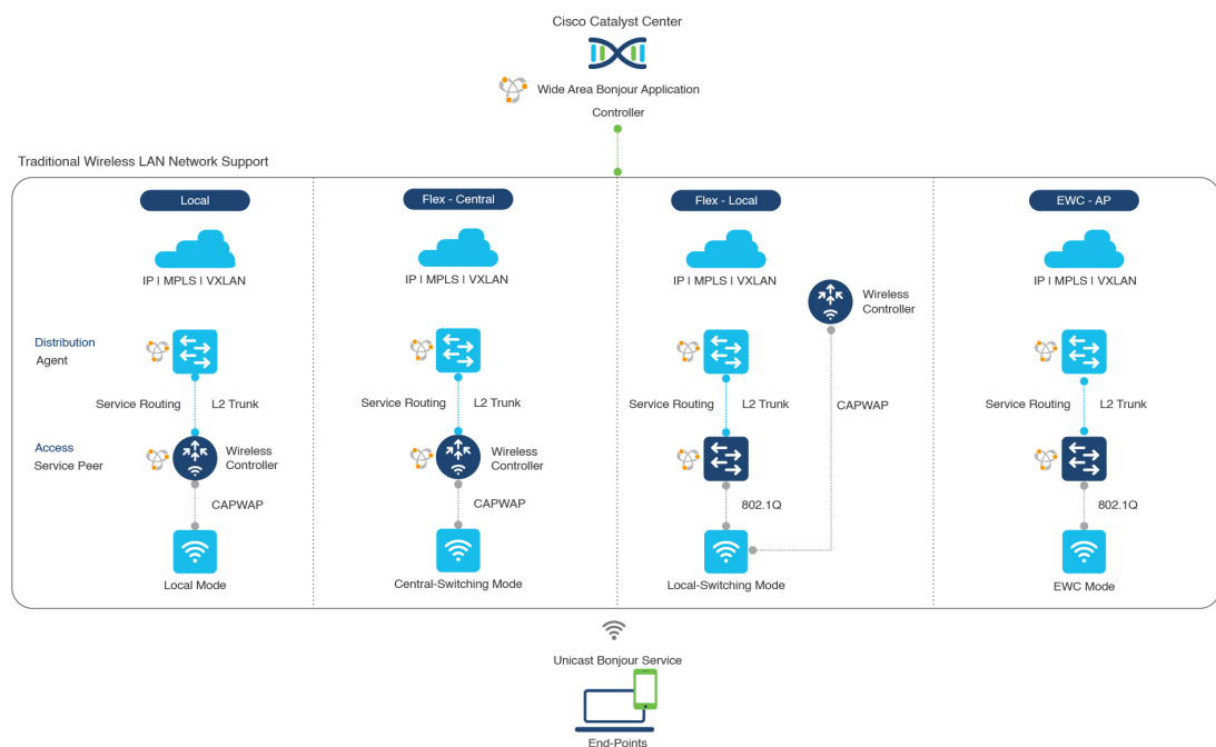
Figure 55: Enterprise Traditional Wireless LAN Network Design
