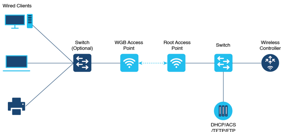
Figure 40: Example of a WGB
