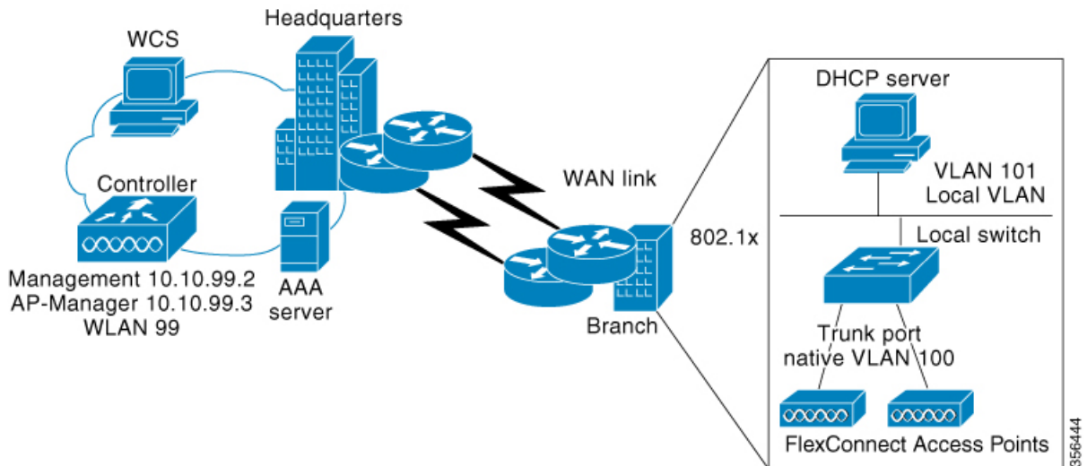
Figure 14: FlexConnect Deployment
