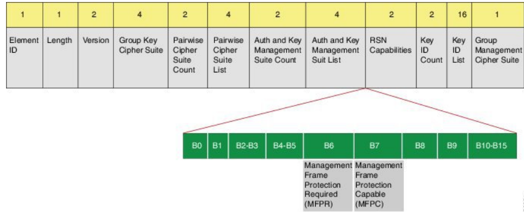
Figure 36: 802.11w Information Elements
