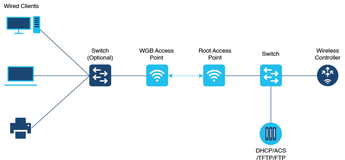
Figure 31: Example of a WGB
