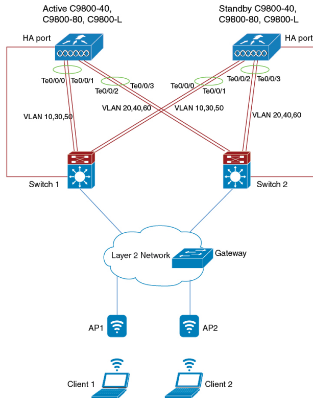
Figure 40: SSO Pair with Multi-LAG
