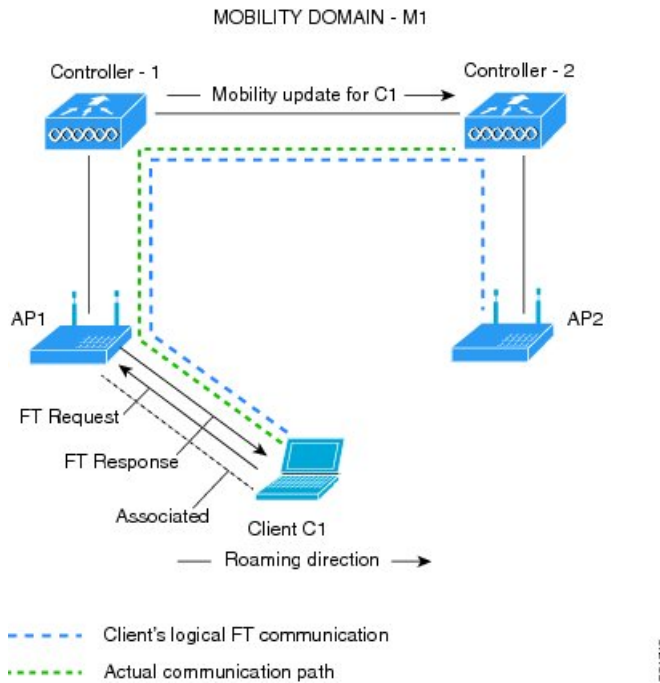
Figure 34: Message Exchanges when Over-the-DS Client Roaming is Configured
