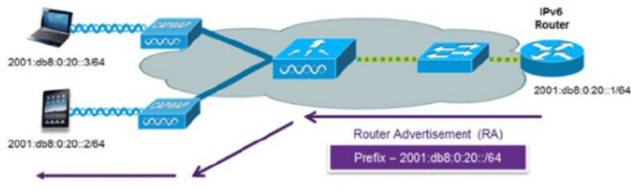
Figure 24: Address Assignment Using SLAAC
