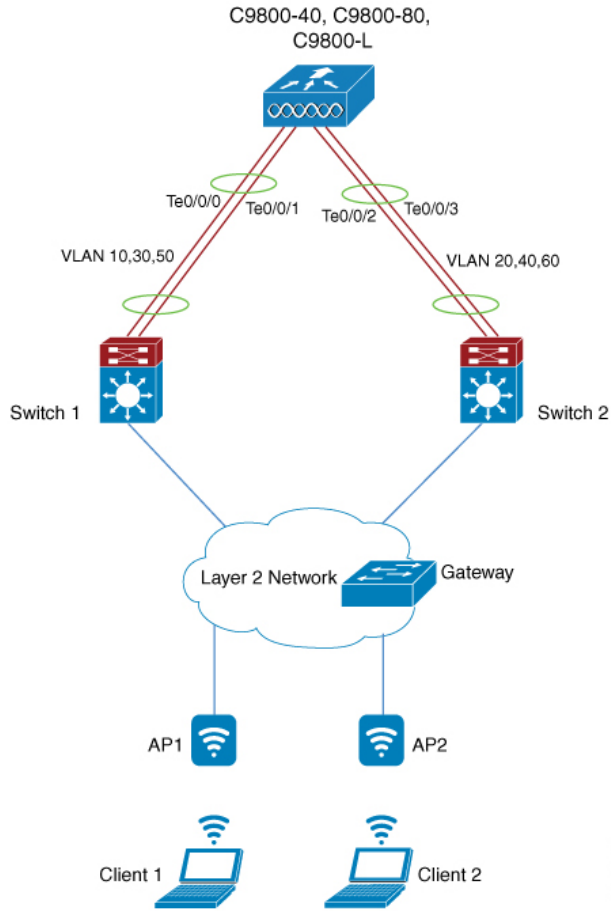
Figure 39: Single Controller with Multi-LAG
