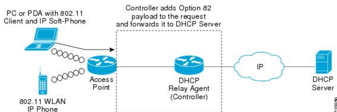
Figure 28: DHCP Option 82
