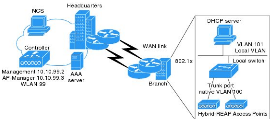
Figure 1: FlexConnect Deployment
