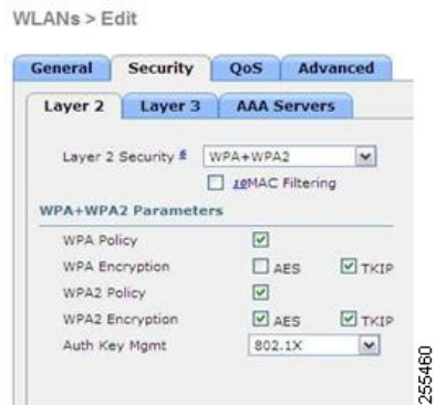
Figure 6: Incompatible WPA and WPA2 Security Encryption Settings for OEAP 600 Series
