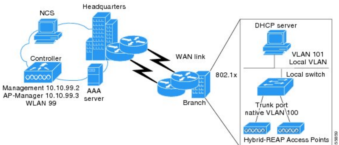
Figure 1: FlexConnect Deployment
