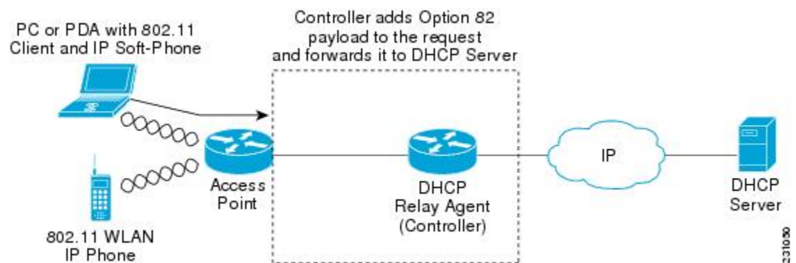
Figure 1: DHCP Option 82
