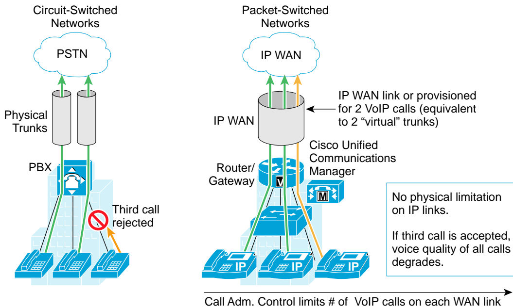
Figure 55 Traditional Versus VoIP Call Admission Control
