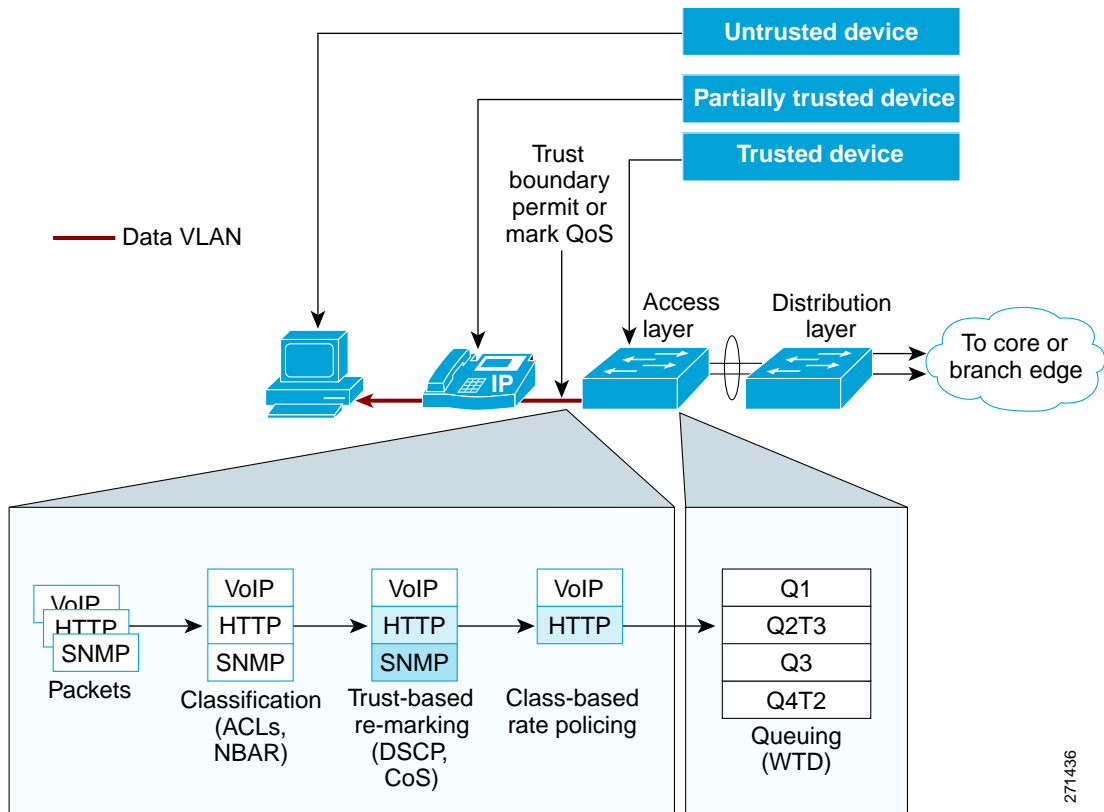
Figure 34 LAN Switch
