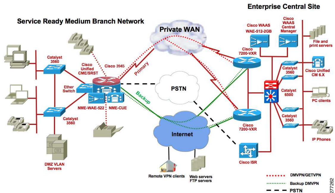
Figure 1 Services Ready Medium Branch Network Test Bed
