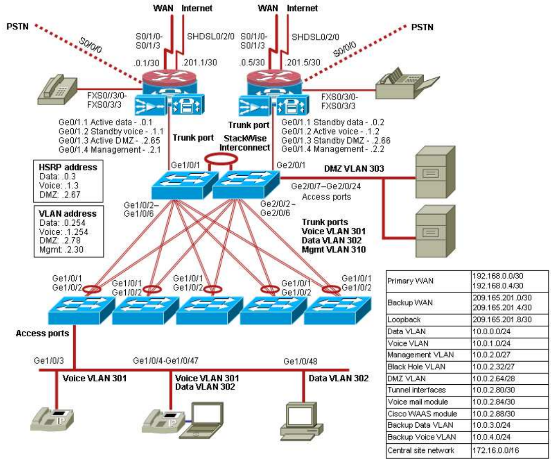
Figure 2 Services Ready Large Branch Network Topology
