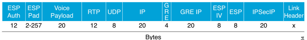
Figure 49 RTP Packet for G.729a Codec with DMVPN Encapsulation
