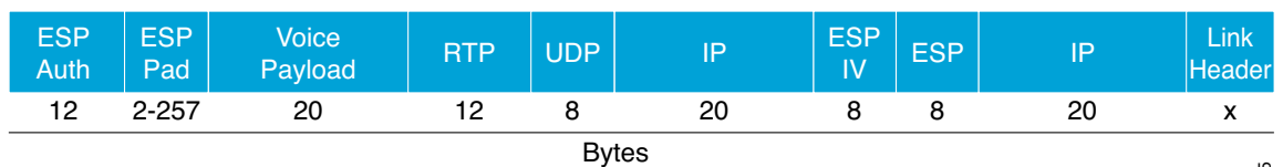
Figure 50 RTP Packet for G.729a Codes with GETVPN Encapsulation
