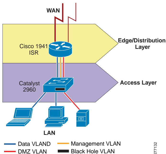
Figure 27 VLAN Design
