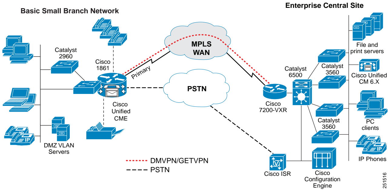
Figure 4 Cisco 1861 ISR MPLS WAN, Cisco Unified SRST Mode
