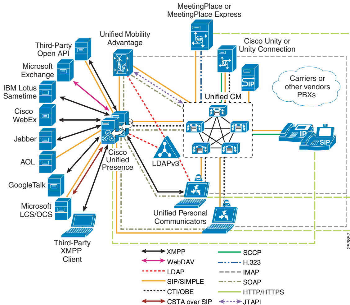
Figure 23-1 Cisco Unified Presence Components
