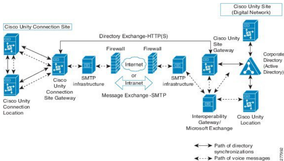
Figure 3: Cisco Voicemail Organization Consisting of a Unity Connection Site Linked to a Cisco Unity Site
