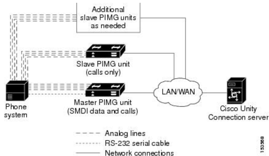
Figure 13: Connections for a Serial (SMDI, MCI, or MD-110) Integration Using Analog PIMG Units
