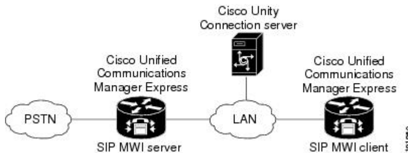
Figure 16: Connections between Multiple Cisco Unified CM Express Routers and a Single Cisco Unity Connection Server
