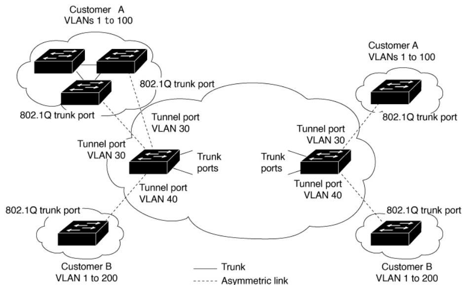
Figure 1: QnQ Topology
