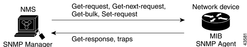
Figure 65-1 SNMP Network
