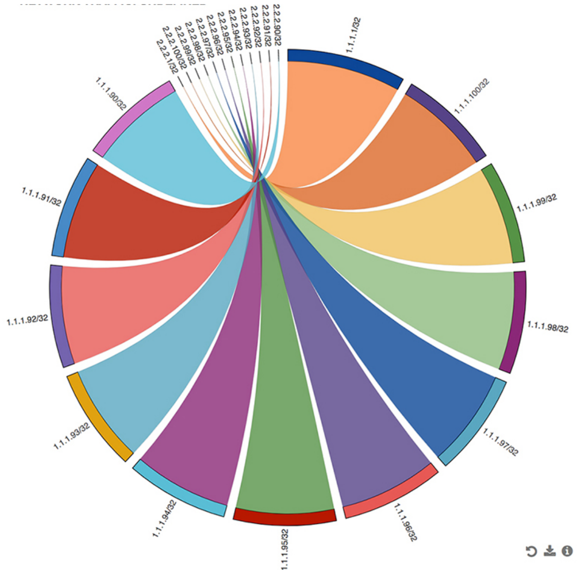
Figure 6: Chord Diagram
