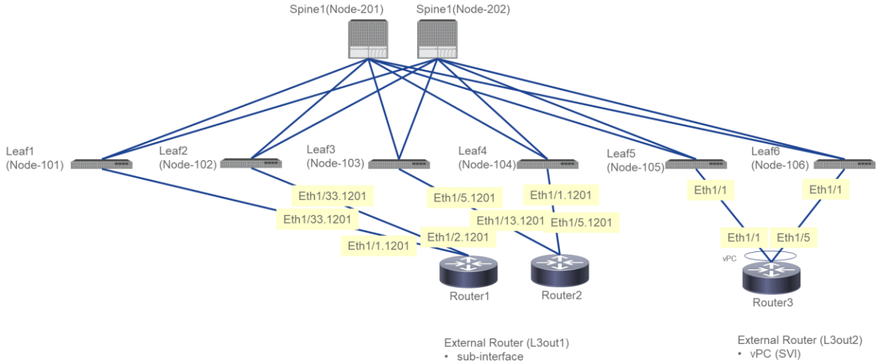
Figure 161. Router2 connectivity
