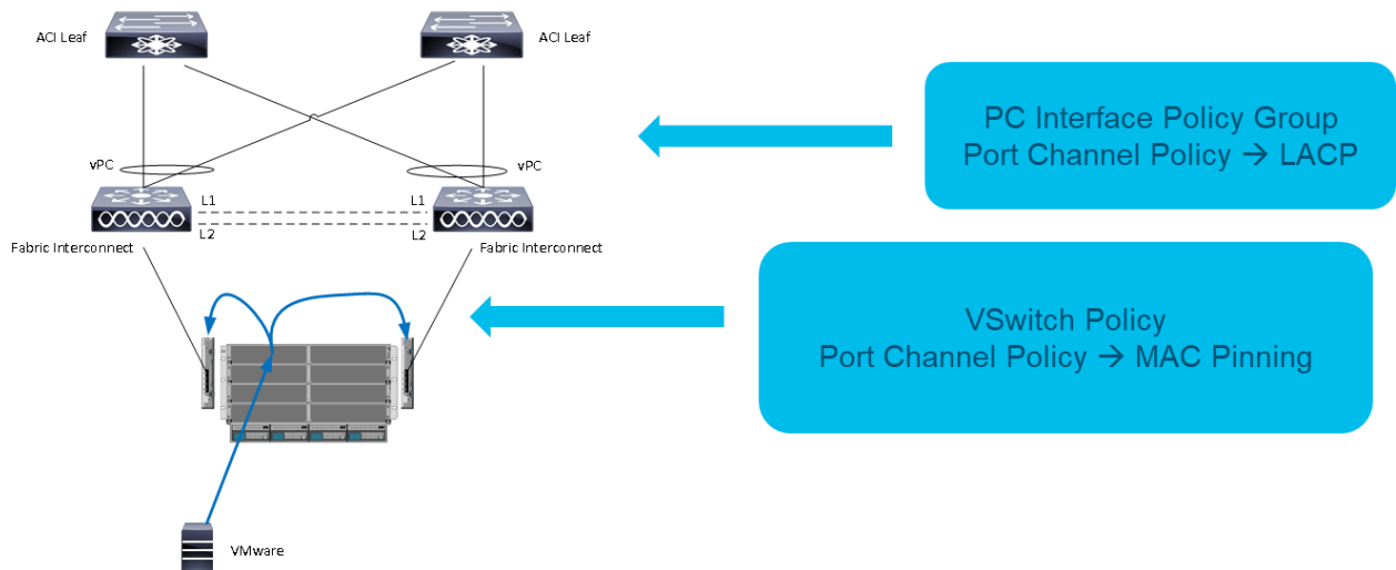
Figure 62. UCS FI blade connectivity
