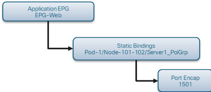
Figure 59. Static Bindings
