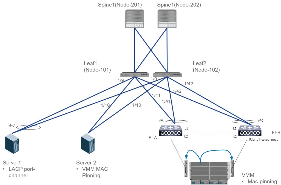
Figure 106. Bare metal with VMM: connectivity
