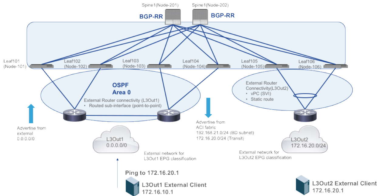
Figure 332. External connectivity
