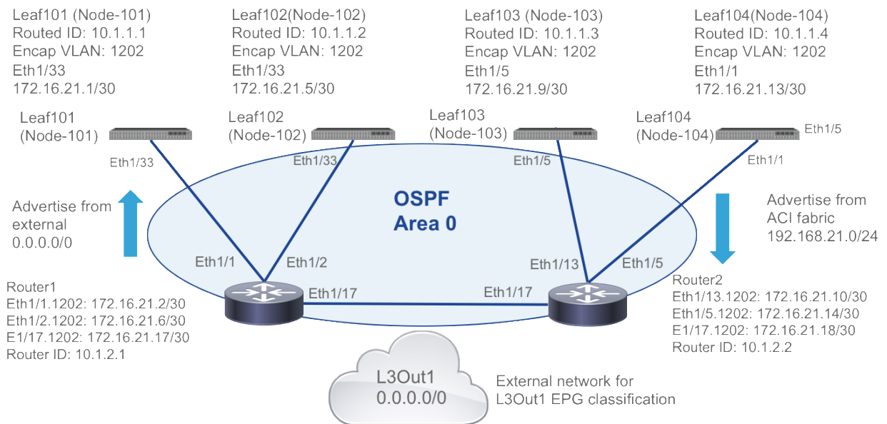
Figure 275. IP addressing
