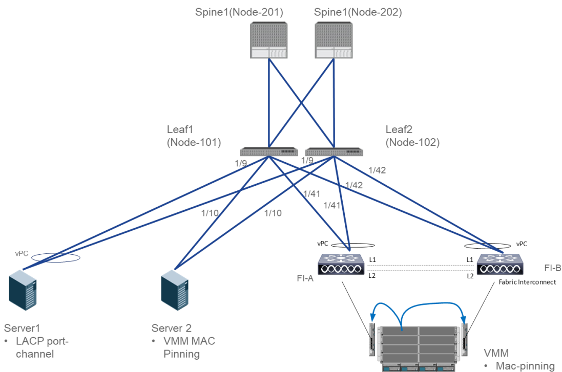
Figure 63. UCS FI blade connectivity in this document
