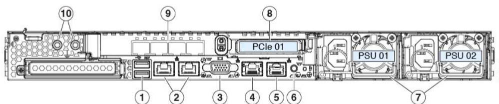
Figure 3. APIC-Server-M3 Rear Interfaces
