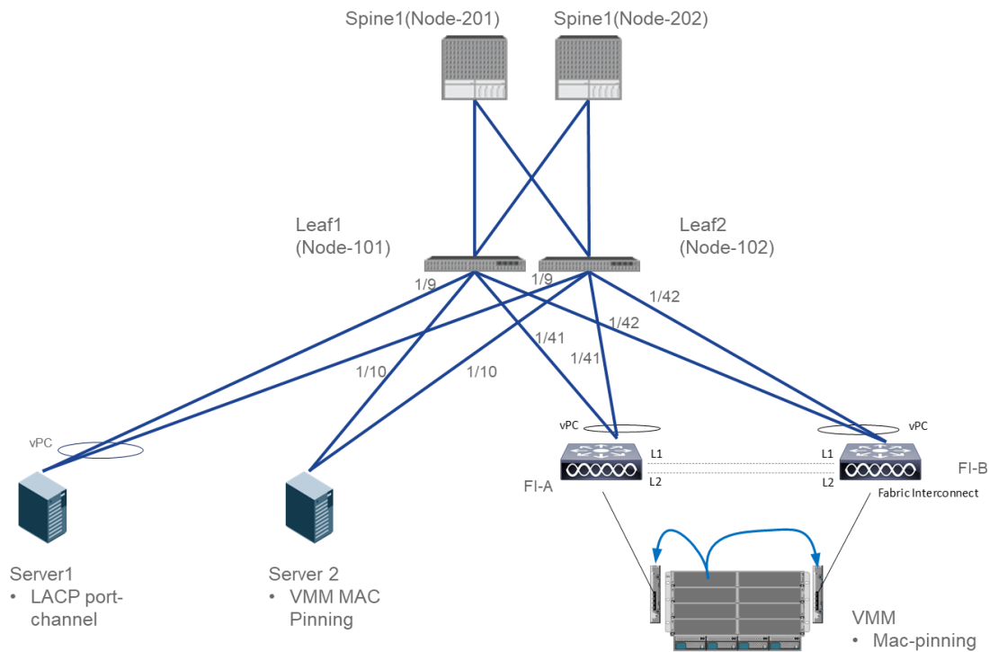
Figure 124. Bare metal with physical domain: connectivity
