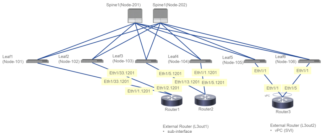
Figure 184. Router3 connectivity
