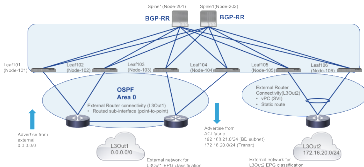
Figure 305. External connectivity
