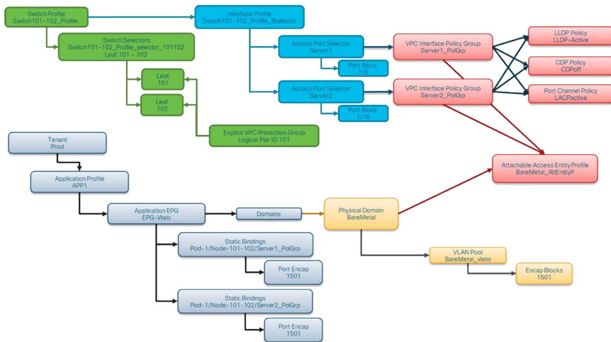
Figure 61. Connecting server1 into our setup
