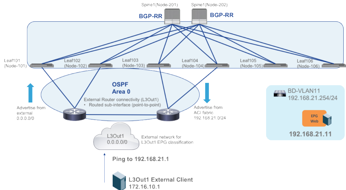
Figure 302. External connectivity
