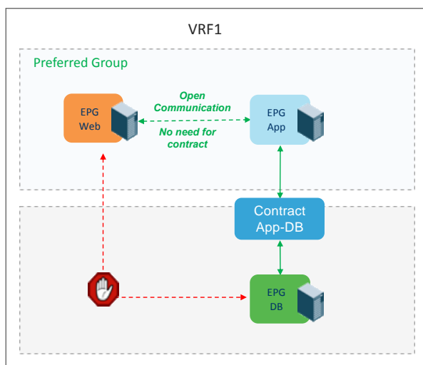
Figure 272. Communication relationship among the three EPGs in App1
