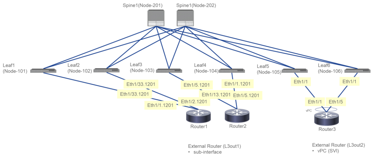
Figure 143. Router1 connectivity
