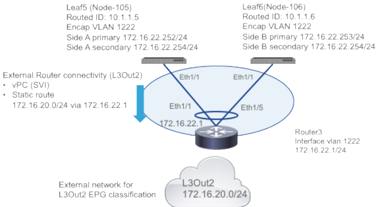
Figure 306. IP addressing
