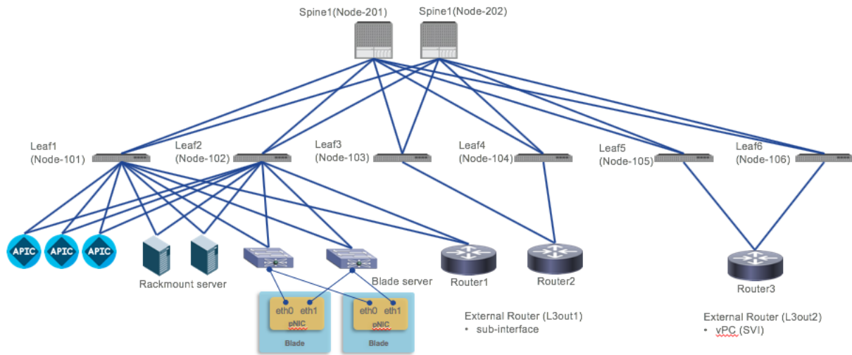
Figure 1. Cisco ACI Topology
