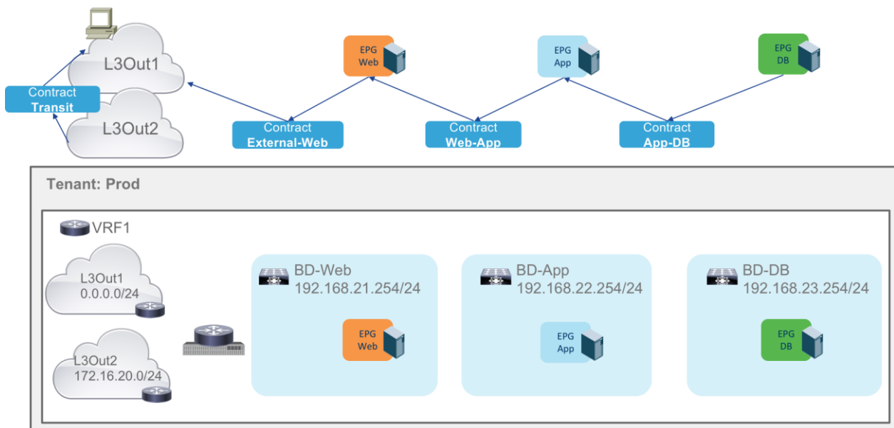
Figure 304. Transit L3out
