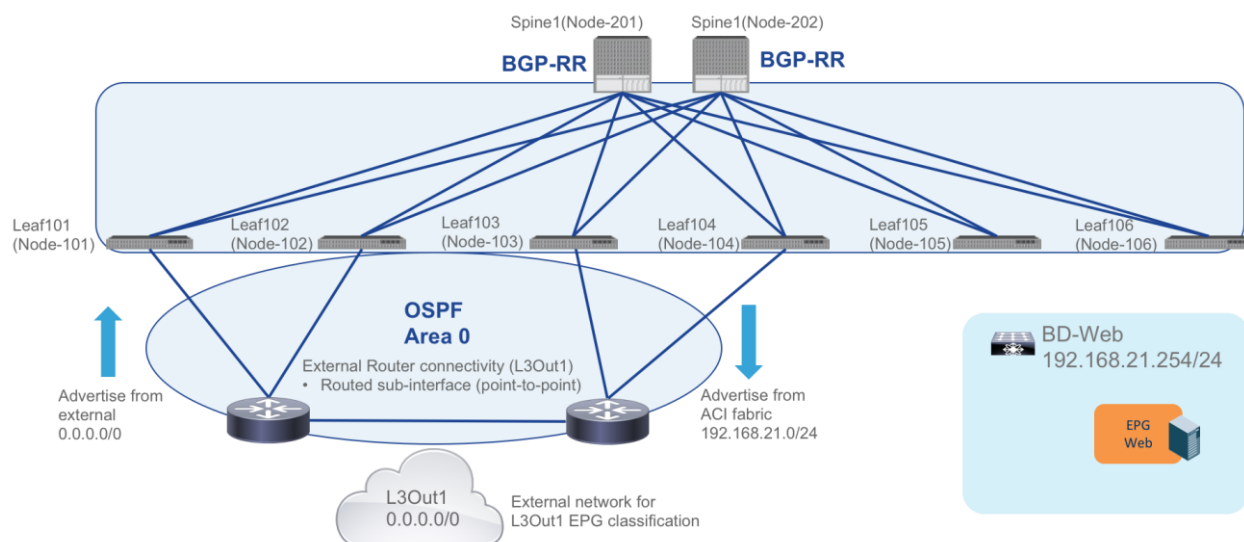
Figure 274. External connectivity
